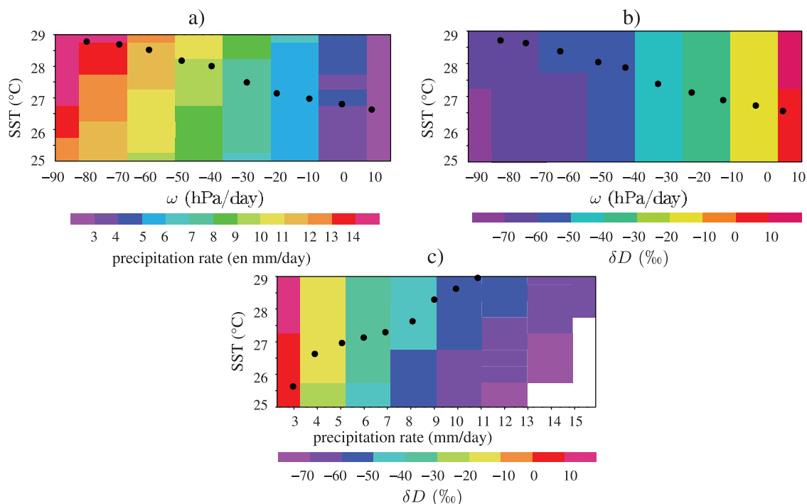
Figure 3. (a) Precipitation (in \text{mm d}^{-1} ) simulated for different conditions of SST and large-scale forcing ( \omega ). The black dots show the mean statistical relationship between SST and \omega derived from reanalysis data [Bony et al. , 2004]. (b) Same as 3a but for \delta D in precipitation. (c) The \delta D in precipitation (in %) presented as a function of SST and precipitation. The black dots show the mean statistical relationship between SST and precipitation rate derived from the black dots of Figure 3a.
