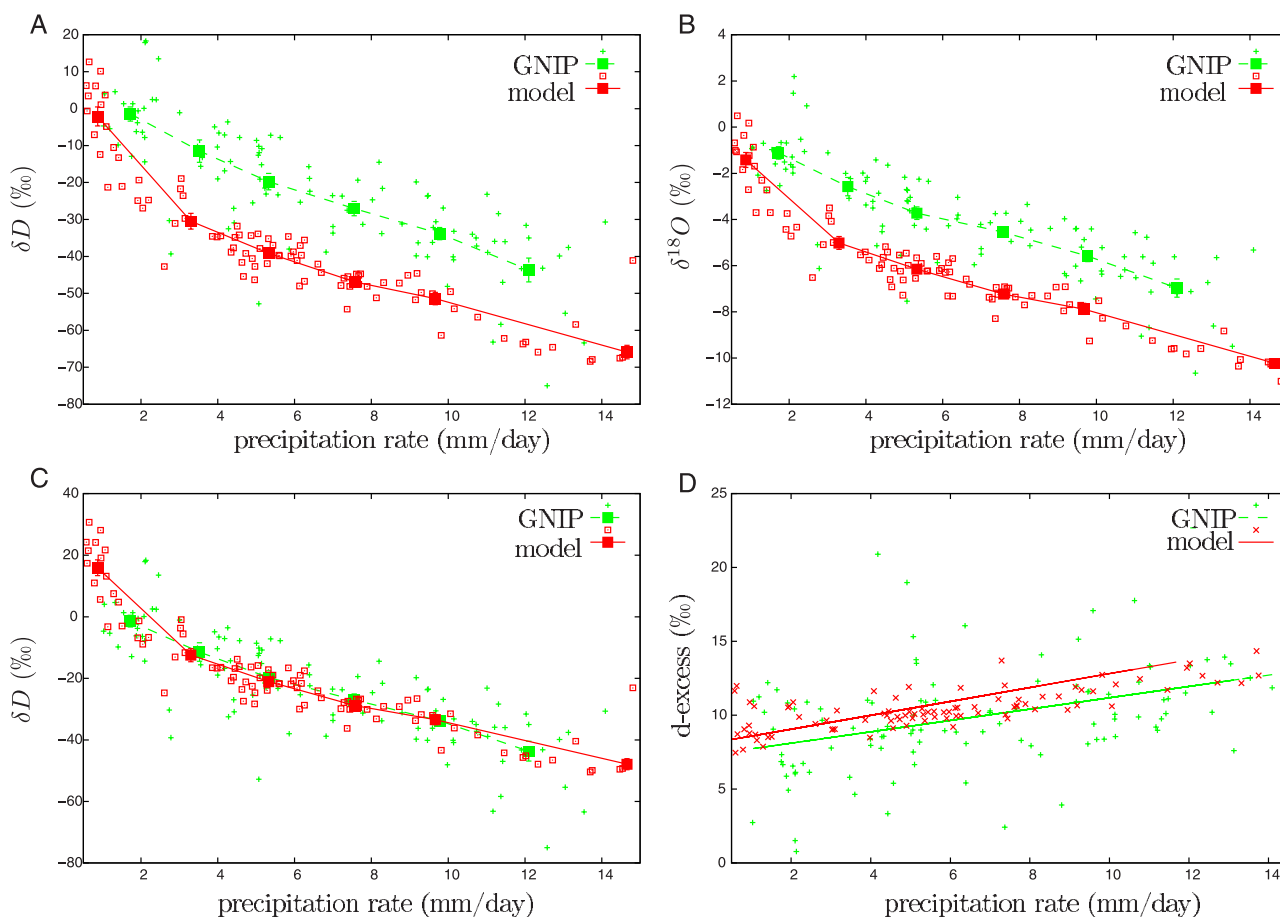
Figure 2. (a) Relationship between monthly values of \delta D in precipitation and the precipitation rate simulated by the single-column model (solid red line) or derived from the GNIIP database (dashed green line) for nine tropical marine stations maintained by the IAEA. Small markers show individual monthly results from observations or simulations. Also reported is the mean relationship between \delta D and precipitation binned into six bins of precipitation rate values. (b) Same as Figure 2a, but for \delta^{18}O . (c) Same as Figure 2a, but after having added an offset of 18‰ to the simulated \delta D to make the comparison between simulations and observations easier. (d) Relationship between the monthly Deuterium excess ( d ) in precipitation and the precipitation rate. Also reported are linear regression lines associated with simulations (thick red) and observations (thin green).
