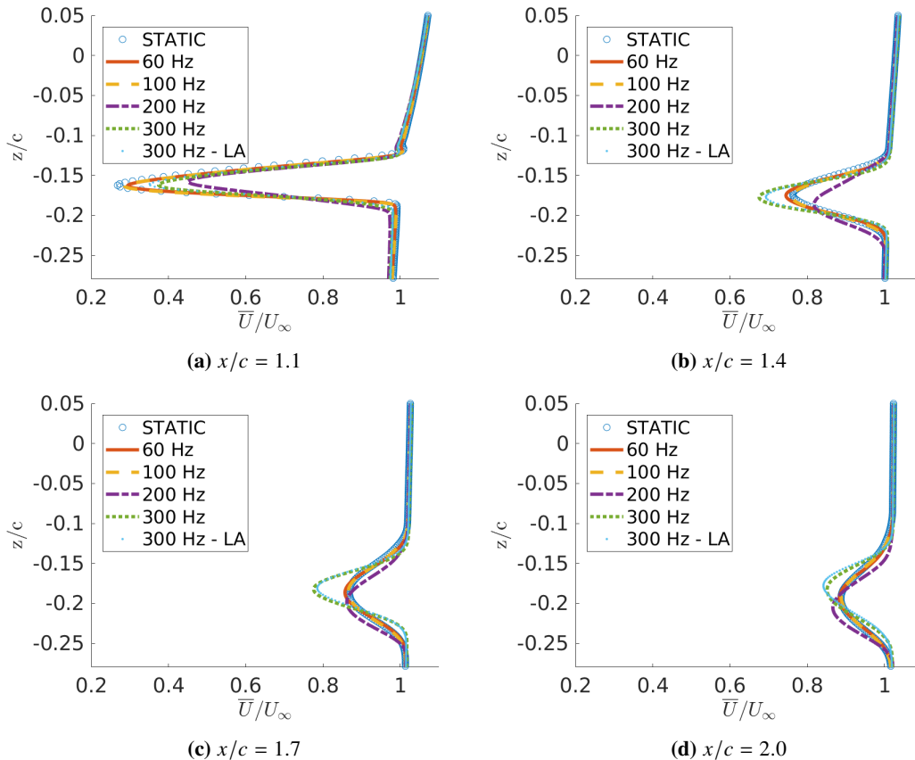
Fig. 10 Comparison of mean longitudinal velocity profiles along the wake for various actuating frequencies; the amplitude is set at 0.35\text{mm} for every morphing application, except for the 300\text{Hz-LA} (lower amplitude) case where a value of 0.15\text{mm} was used.
