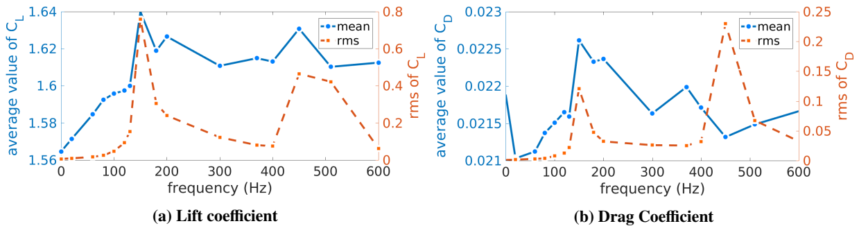
Fig. 11 Effect on the aerodynamic coefficients versus frequency variations with a constant amplitude of 0.35\text{mm} ; zero values for frequency imply absence of morphing.
