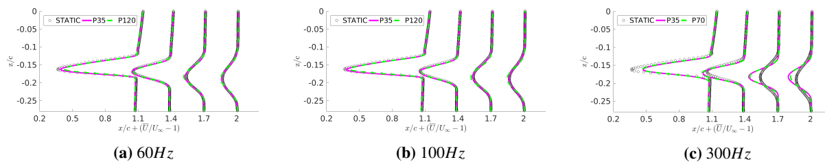
Fig. 12 Comparison of mean longitudinal velocity profiles along the wake for various L_p patch lengths; the amplitude is set at 0.35\text{mm} for every morphing application.
