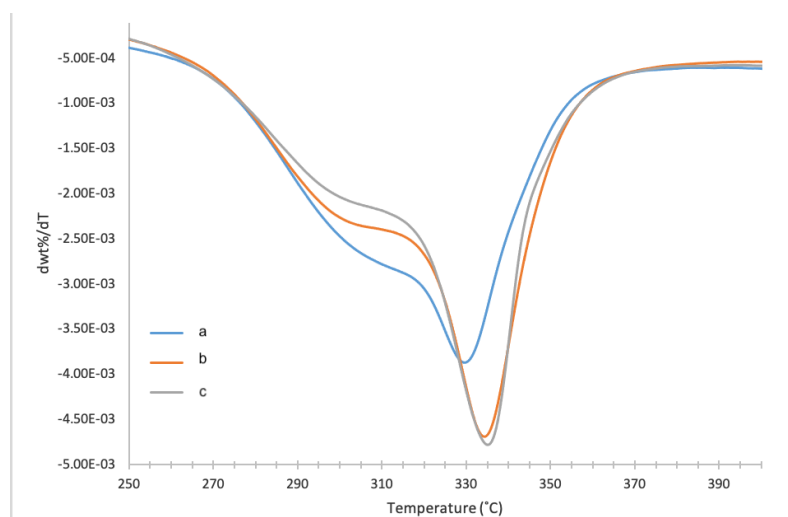
Fig. 1 : Derivative of thermogravitation curves (DTG) of oak samples heated from 50 °C to 800 °C at 20 °C/min under air. The concentration of natural potassium in the samples is as follows: (a) [K] = 0.1657%, (b) [K] = 0.1039%, and (c) [K] = 0.0707%.
