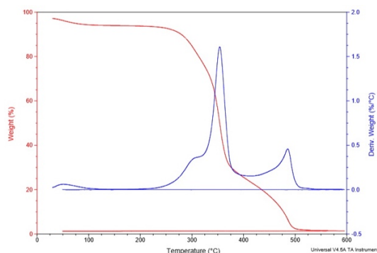
Fig. 2: TG & DTG curve of Kenaf
