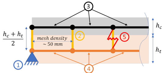
Fig. 3: Composite beam FEM model: (1) support; (2) vertical strut elements, rigid in terms of axial stiffness; (3) concrete elements; (4) timber elements; (5) horizontal connector elements, a spring element with defined horizontal stiffness (connector stiffness)
