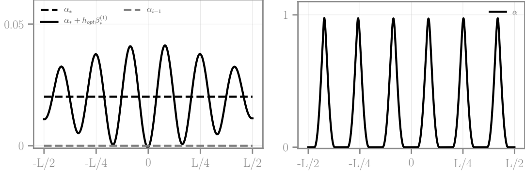
Figure 11: Left : Detail of the bifurcation at the onset of damage, showing the unstable homogeneous state \alpha_* , the irreversibility lower bound \alpha_{i-1} and the optimally perturbed state \alpha_* + h_{opt}\beta^{(1)} , see Algorithm 3. Right: Fully localised solution for the damage field \alpha obtained at the end of the simulation.
