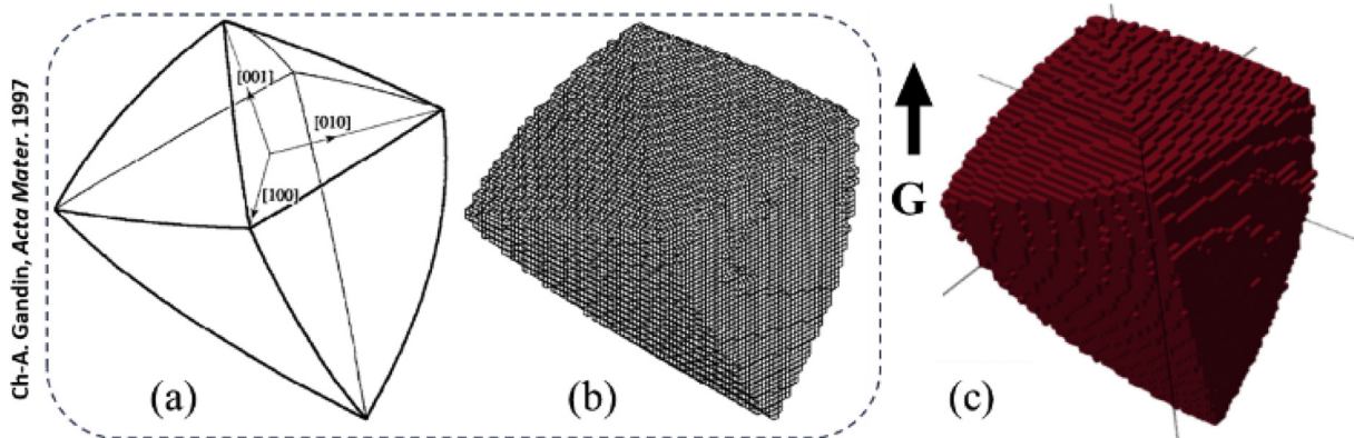
Fig. 8. Results of monocrystal growth obtained by Gandin et al. [44] (a) analytically and (b) numerically, and (c) obtained numerically using the model presented in this study.
