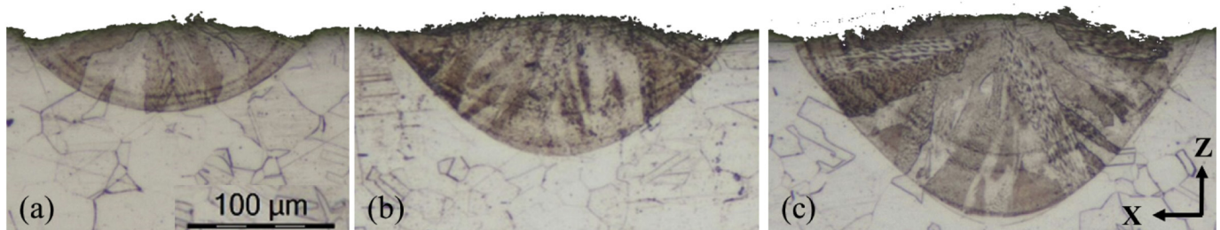
Fig. 10. Cross sections of fusion lines obtained with various power and travel speed: (a) P1, 320 W - 400 \text{mm.s}^{-1} , (b) P2, 400 W - 400 \text{mm.s}^{-1} , (c) P3, 400 W - 310 \text{mm.s}^{-1} .
