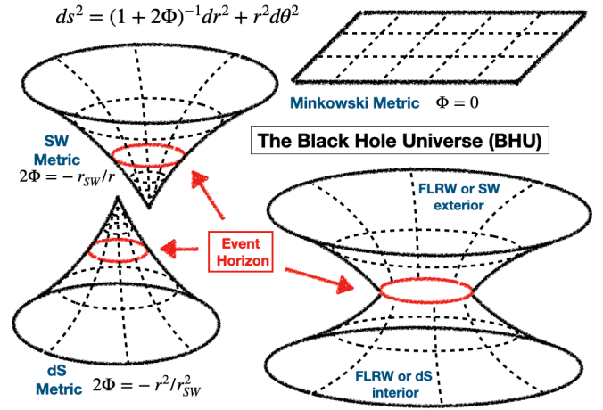
Figure 5. Time slice ( dt = 0 ) representation of ds^2 = (1+2\Phi)^{-1}dr^2 + r^2d\theta^2 (polar coordinates) for Minkowski ( \Phi = 0 , flat), BH.SW ( 2\Phi = -1/r , singular at r = 0 ), and dS ( 2\Phi = -r^2 , singular at r = \infty ) metrics. The dashed lines also correspond to geodesics or particle orbits. The BHU classical solution to GR has two nested FLRW metrics and no singularities. Note how this is very different from joining the BH.SW and dS metrics at the singularity which is not a solution to classical GR.
