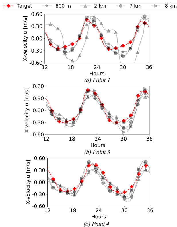
Figure 12- Example of optimal calibration with the tested domain extents, for x-velocity u at points 1, 3 and 4.
