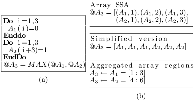
Figure 2: (a) Sample code in Array SSA form (not all gates shown for simplicity). (b) Array SSA forms: (top) as proposed by [16], (center) with reduced accuracy and (bottom) using aggregated array regions.
