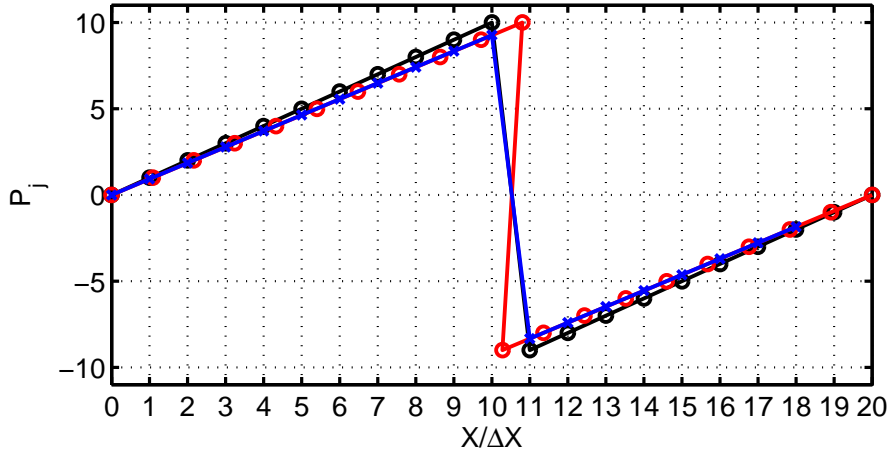
Fig. 3 Example of calculation between two time steps. Black: solution at time step n with pressure values P_j^n at the grid points X_j . Red: solution at the time step n + 1 based on the pressure values P_j^n at the points Y_j (note the multi-valued region at the shock). Blue: actual solution at time n + 1 with pressure values P_j^{n+1} at grid points X_j .
