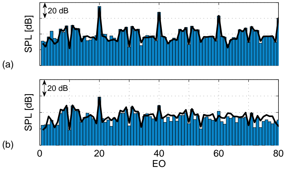
Fig. 18 Comparison between numerical results from the 1DNP-TFD code and measured data at (a) station 1 and (b) station 3. EO frequency spectrum in the rigid intake duct. Key: Black line—1DNP-TFD; Blue bars—data.
