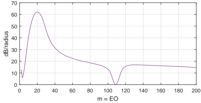
Fig. 11 Linear decay rates for engine orders 1 to 100.
