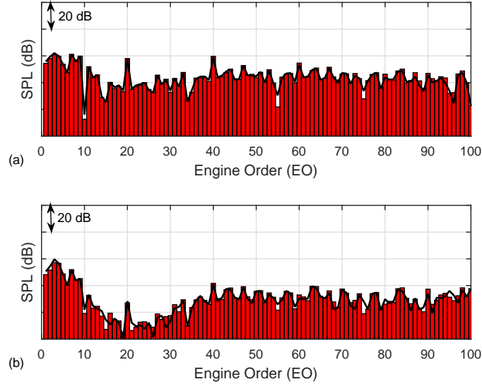
Fig. 15 Comparison between numerical results from the FDNS and 1DNP-TFD codes. EO frequency spectrum for irregular sawtooth \underline{IR}_2 in a lined cylindrical intake duct: (a) z/D = 0.25 , and (b) z/D = 0.5 . Key: Red bars—FDNS; Black line—1DNP-TFD.
