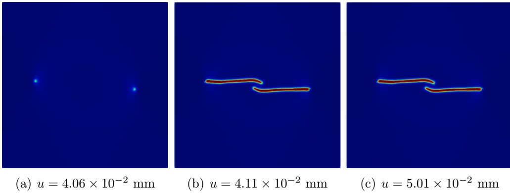
Figure 10: Crack evolution in the double notched tensile specimen
