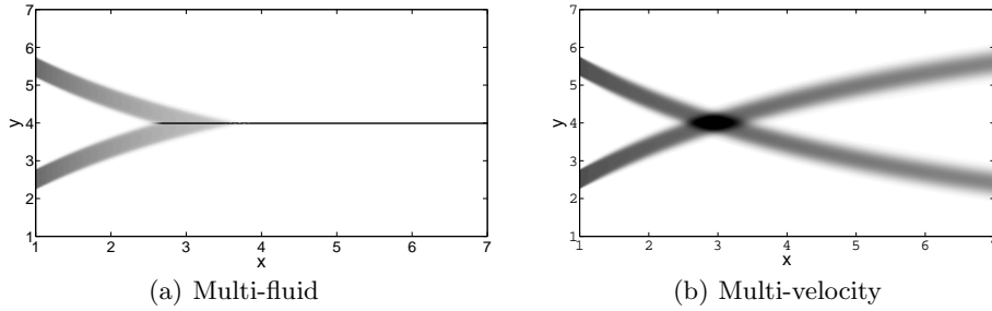
FIGURE 2. Mass density for simulation of two crossing jets using the standard multi-fluid approach (left) and the multi-fluid/multi-velocity model (right) for droplets with St = 5.29 .
