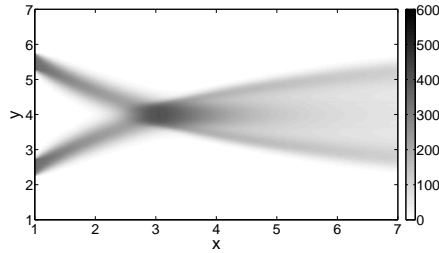
FIGURE 6. Mass density for the simulations of two crossing jets using the BGK model with multi-fluid multi-velocity model for droplets with St = 5.29 undergoing collisions.
