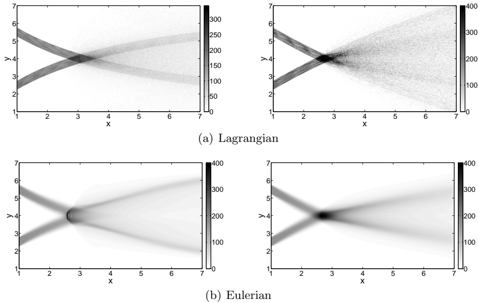
FIGURE 7. Mass density for the simulations of two crossing bi-disperse jets using the DPS approach averaged and projected onto the Eulerian grid (a) and the multi-fluid/multi-velocity model (b). Droplets of Stokes number St = 5.29 are represented on the left side and droplets of Stokes number St = 15.86 are represented on the right side
