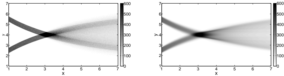
FIGURE 3. Mass density for the simulations of two crossing monodisperse jets using the DPS approach averaged and projected onto the Eulerian grid (left) and the multi-fluid/multi-velocity model (right) for droplets with St = 5.29 undergoing collisions.
