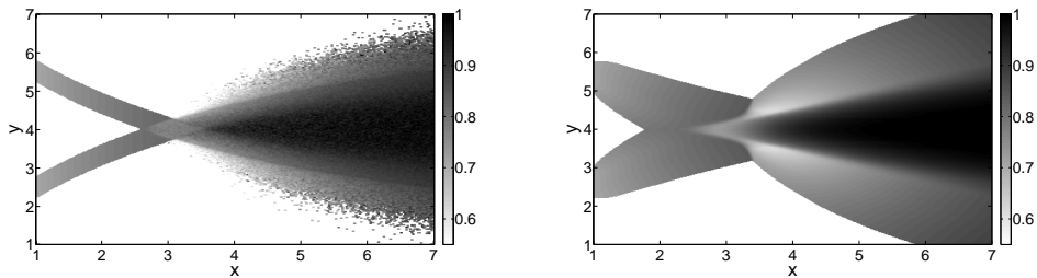
FIGURE 4. Mean particle velocity in the x -direction for the simulations of two crossing monodisperse jets using the DPS approach averaged and projected onto an Eulerian grid (left) and the multi-fluid/multi-velocity model (right) for droplets with St = 5.29 undergoing collisions.
