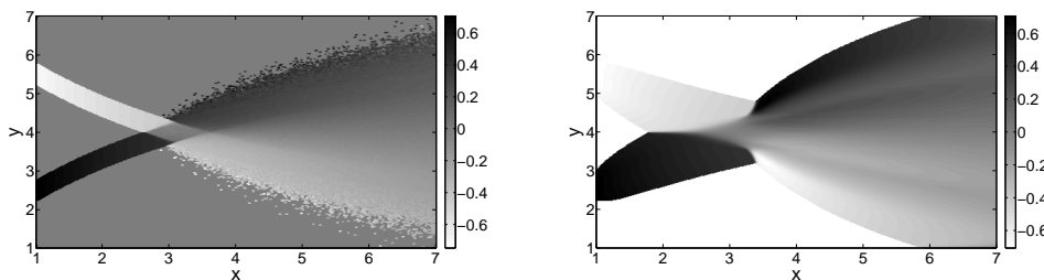
FIGURE 5. Mean particle velocity in the y -direction for the simulations of two crossing monodisperse jets using the DPS approach averaged and projected onto an Eulerian grid (left) and the multi-fluid/multi-velocity model (right) for droplets with St = 5.29 undergoing collisions.
