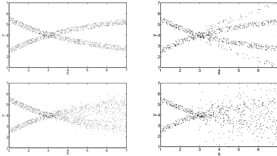
FIGURE 1. Droplet positions in the Lagrangian simulation without collision (top) and with collisions (bottom) for the monodisperse case (left) and the bi-disperse case (right).
