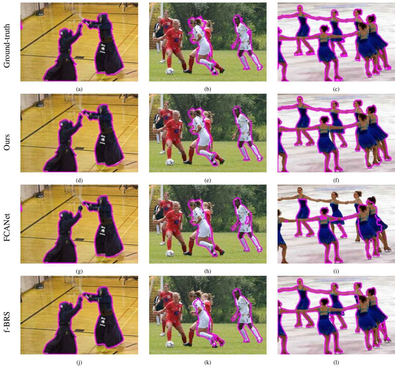
Figure 6: The magenta boundaries delineate regions with foreground labels for the ground-truth data, our method, and the baselines using 5 clicks per image on the iCoSeg dataset. Figure (i) shows that FCANet has difficulties when segmenting multiples instances, as mentioned in their original article.
