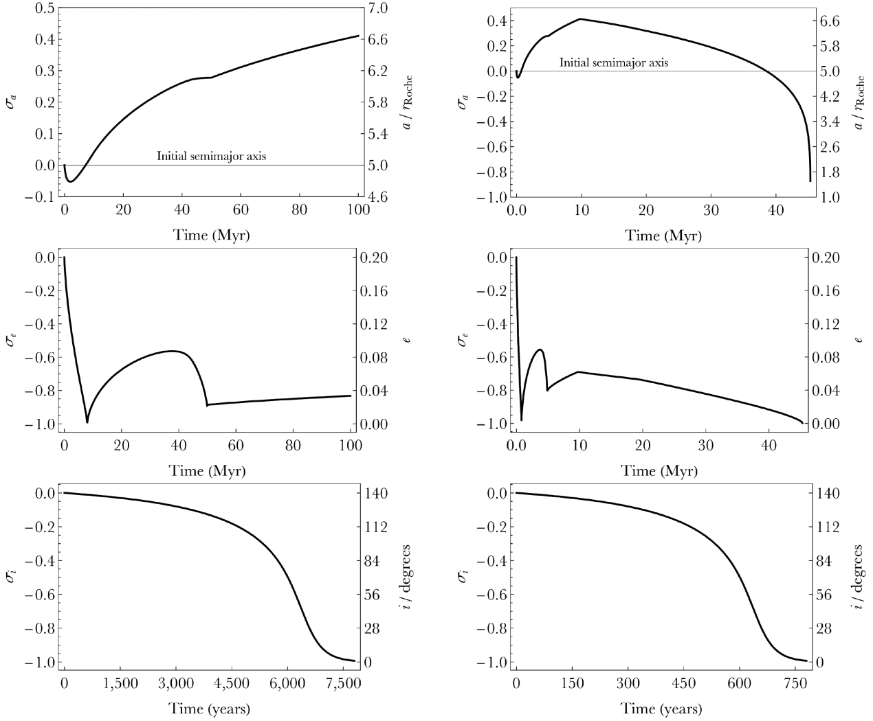
Figure 1. Two examples (left-hand and right-hand panels) of the orbital evolution of a planet tidally interacting with a white dwarf, where definitions of \sigma_a , \sigma_e , and \sigma_i are given in equations (14)–(16). In both examples, a(0) = 5r_{\text{Roche}} , e(0) = 0.20 , M = 10M_{\oplus} , \rho = \rho_{\oplus} , and (d\theta/dt)(0) = 360^\circ/(20 \text{ h}) . In the left-hand panels, \eta = 10^{20} \text{ Pa}\cdot\text{s} , whereas in the right-hand panels, \eta = 10^{19} \text{ Pa}\cdot\text{s} ; i.e. the only difference in the simulations is a one order of magnitude variation in the planetary viscosity. In the left-hand panels, over 100 Myr, the semimajor axis evolution is increased overall, but in a non-uniform manner and only after shifting direction. In contrast, in the right-hand panels, the planet changes direction twice, and is eventually destroyed by entering the Roche radius after 54 Myr. In both panels, the initial inclination of the orbit i(0) = 140^\circ with respect to the planet’s equator is quickly reduced to within 1^\circ . The damping of i' (inclination with respect to the stellar equator) is even quicker (note the different scales of the time axes).
