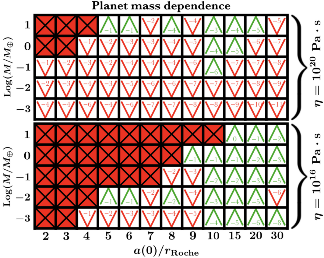
Figure 3. Same as Fig. 2 but for planet mass dependence, and assuming \rho = \rho_{\oplus} in all cases, with \eta = 10^{20} \text{ Pa} \cdot \text{s} for the top panel and \eta = 10^{16} \text{ Pa} \cdot \text{s} for the bottom panel. The final outcome is strongly dependent on planetary mass.
