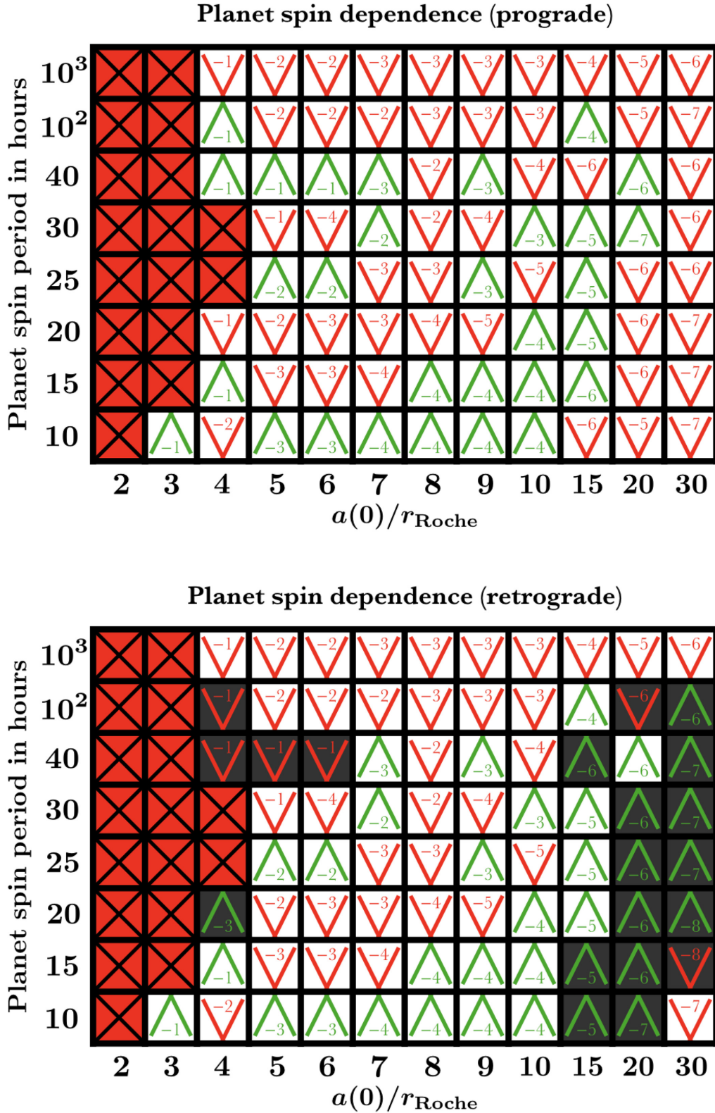
Figure 4. Same as Fig. 2 but for planetary spin period dependence, and assuming \eta = 10^{20} Pa·s. The upper grid gives results for prograde planetary spins (relative to orbit orientation), and the bottom grid for retrograde planetary spins. The grids are 79 per cent coincident; grey squares in the bottom grid locate the discrepancies. The final outcome has a complex dependence on planetary spin period.
