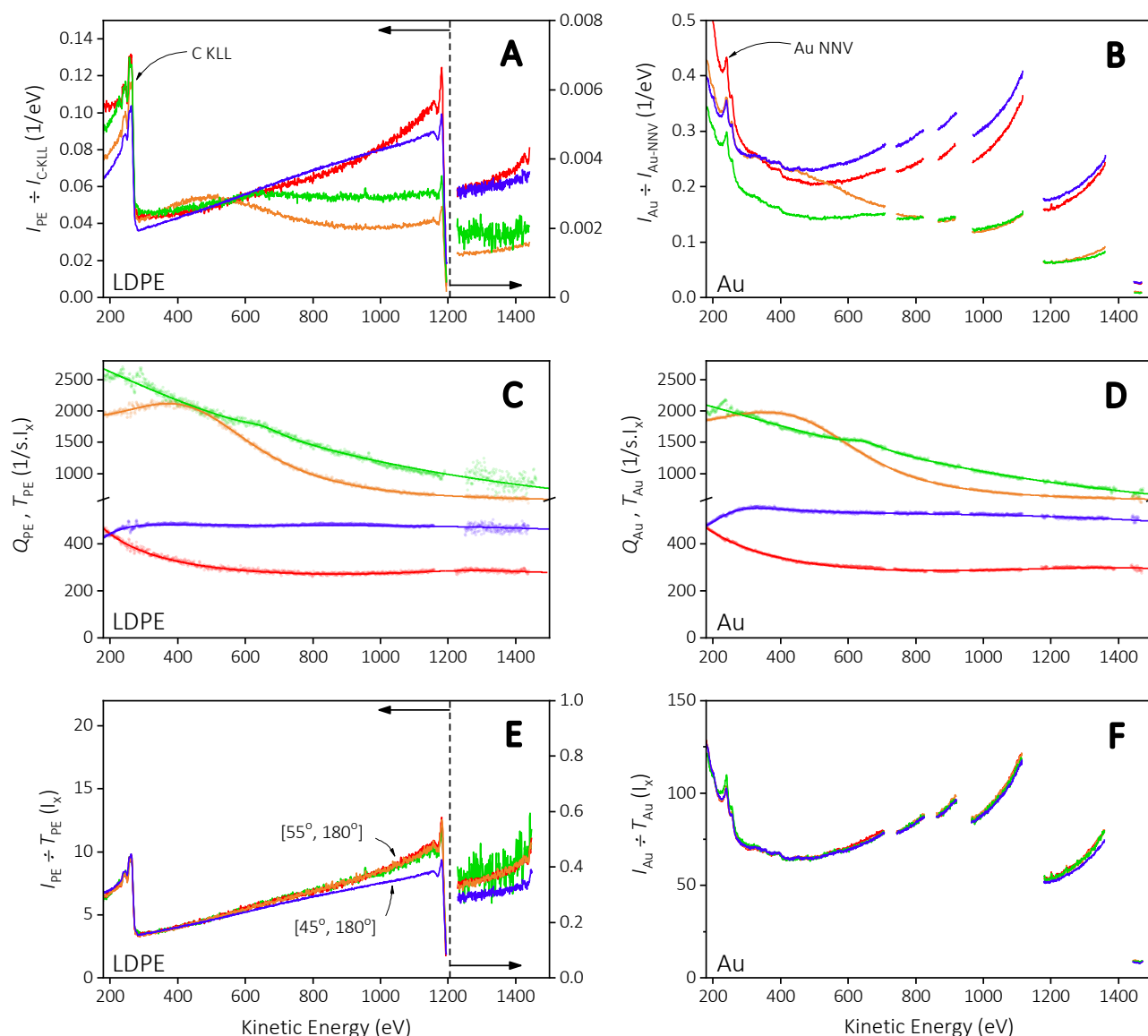
FIG. 2. Transmission function correction using LDPE and Au spectra from participants AX (red), AJ (blue), AI (green), and AT (orange). (A, B) LDPE and Au spectra normalised to the C KLL and Au NNV Auger peaks respectively. (C, D) Q (dots) and T (lines) calculated using LDPE and Au intensity calibration methods respectively. (E, F) Intensity-corrected LDPE and Au spectra using T_{PE} and T_{Au} respectively.
