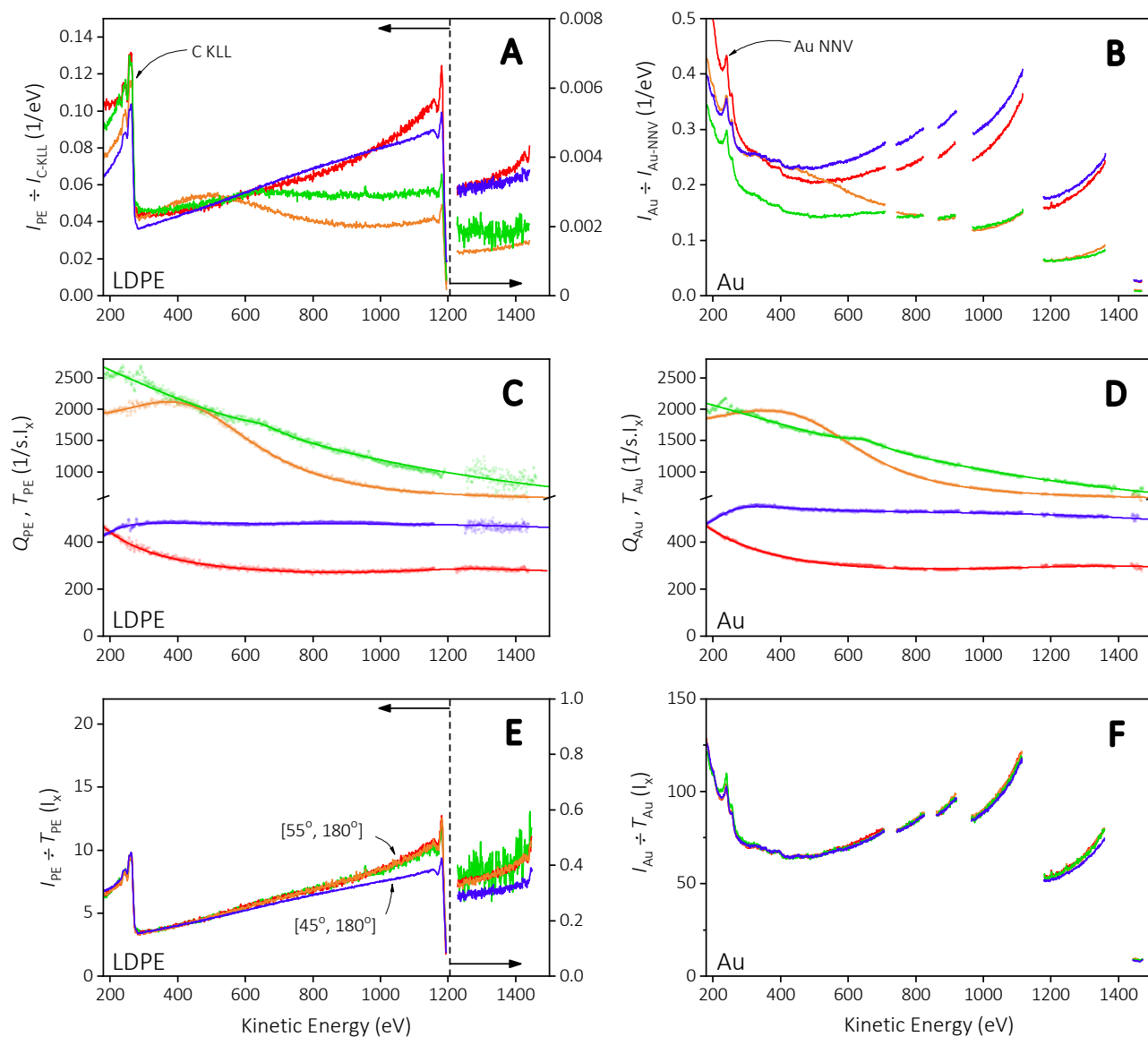
FIG. 2. Transmission function correction using LDPE and Au spectra from participants AX (red), AJ (blue), AI (green), and AT (orange). (A, B) LDPE and Au spectra normalised to the C\ KLL and Au NNV Auger peaks respectively. (C, D) Q (dots) and T (lines) calculated using LDPE and Au intensity calibration methods respectively. (E, F) Intensity-corrected LDPE and Au spectra using T_{PE} and T_{Au} respectively.
