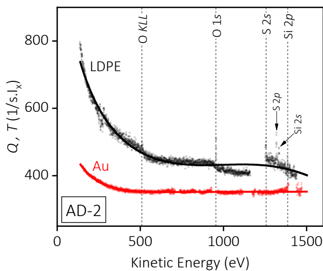
FIG. 7. Q_{PE} and Q_{Au} from participant AD-2 demonstrating the significant effect that contamination on the LDPE produces. Other elements (i.e. O, Si, and S) on the LDPE cause steps, discontinuities, and deviations in Q_{PE} .
