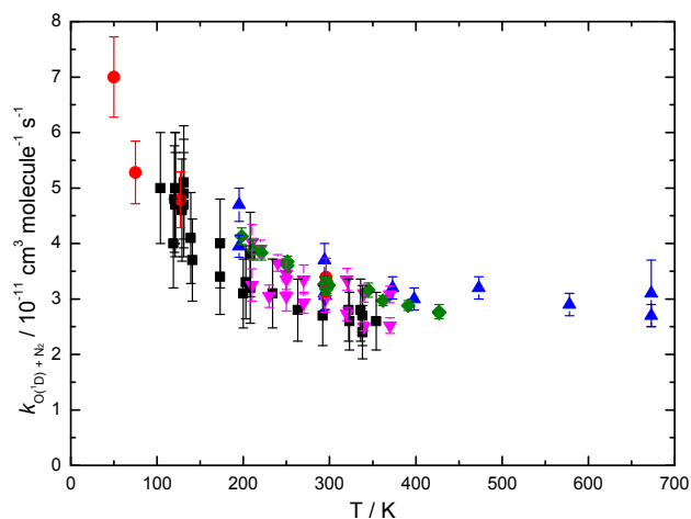
Figure 4 Rate constants for the O( 1 D) + N 2 reaction as a function of temperature. (Red filled circles) This work; (Black filled squares) Streit et al.; 6 (Blue filled triangles) Blitz et al.; 9 (Pink filled triangles) Dunlea & Ravishankara; 1 (Green filled diamonds) Strekowski et al. 2
