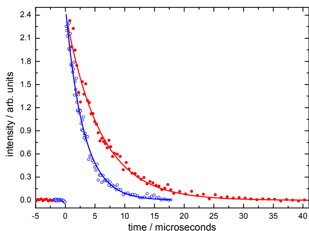
Figure 1 O( 1 D) VUV LIF intensity as a function of time recorded at 50 K. (Red solid circles) O( 1 D) quenching in the presence of the carrier gas Ar alone ( [\text{Ar}] = 2.59 \times 10^{17} molecule \text{cm}^{-3} ); (Blue open circles) O( 1 D) quenching in the presence of the carrier gas Ar ( [\text{Ar}] = 2.59 \times 10^{17} molecule \text{cm}^{-3} ) with added N 2 ( [\text{N}_2] = 2.56 \times 10^{15} molecule \text{cm}^{-3} ).
