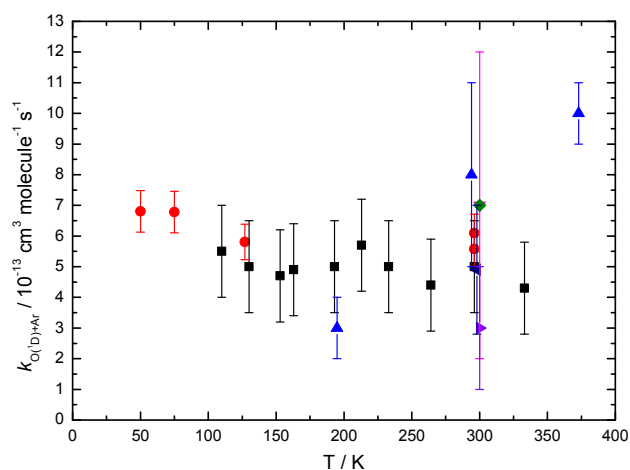
Figure 3 Rate constants for the O(^1D) + Ar reaction as a function of temperature. (Red filled circles) This work; (Black filled squares) Davidson et al.; 22 (Blue filled triangles) Blitz et al.; 9 (Pink filled triangle) Preston & Cvetanovic; 23 (Green filled diamond) Heidner & Husain; 24
