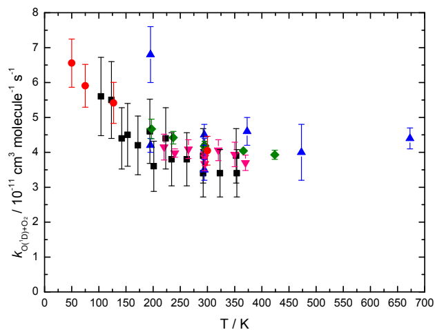
Figure 5 Rate constants for the O( 1 D) + O 2 reaction as a function of temperature. (Red filled circles) This work; (Black filled squares) Streit et al.; 6 (Blue filled triangles) Blitz et al.; 9 (Pink filled triangles) Dunlea & Ravishankara; 1 (Green filled diamonds) Strekowski et al. 2
