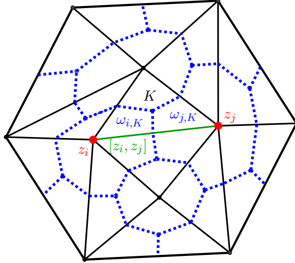
Fig. 2: Triangular mesh \mathcal{T} (solid line) and dual mesh \mathcal{M} (dashed line).
