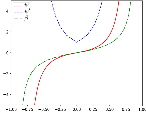
Fig. 1: Functions \psi , \psi' and \beta .
