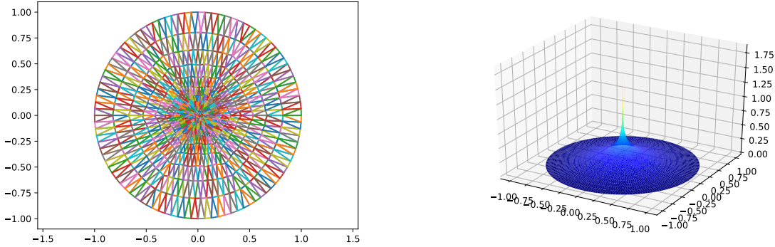
Fig. 4: Domain \Omega and mesh in the case n = 817 (left), numerical solution with n = 12481 (right)
