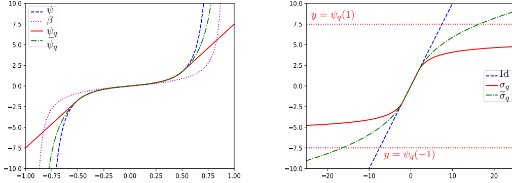
Fig. 3: Left: Functions \psi , \beta , \psi_q and \tilde{\psi}_q with q = \frac{1}{2} . Right: Functions \sigma_q and \tilde{\sigma}_q with q = \frac{1}{2} . The lines y = \psi_q(\pm 1) are the asymptotes of the function \sigma_q at \pm\infty .
