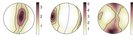
Figure 6. Representative pole figures for crystallographic axes [100], [010], and [001] of olivine (a) and the crystallographic axes or poles [100], (010), and (001) of plagioclase (b) in Wadi Somerah. The pole figures are arranged by their height in the sequence; text block aside gives the layer number and the sample position within the layer (base/top), the depth in the layered sequence, the corresponding BA or BC index, and the ODF J index of the sample. N is the number of analyzed grains. The blue line gives the foliation estimated from (010) of plagioclase. The star behind a layer number indicates a low number of analyzed grains (<70). Patterns with a point of every analyzed pixel are plotted for samples with <70 analyzed grains because contoured pole figures are not significant here. Note the differently scaled color bars.
