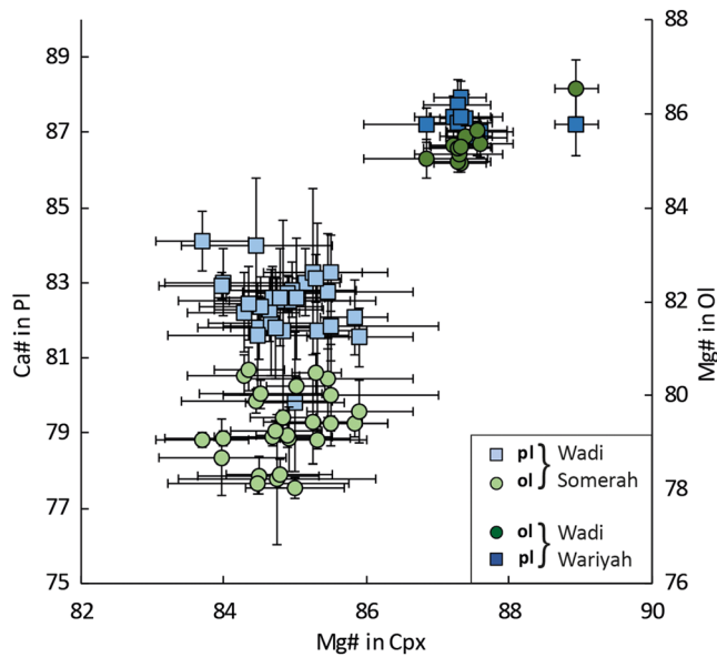
Figure 9. Ca# ( (\text{Ca}/(\text{Ca} + \text{Na}) \times 100 ; molar basis) in plagioclase and Mg# ( (\text{Mg}/(\text{Mg} + \text{Fe}) \times 100 ; molar basis) in olivine plotted versus Mg# in clinopyroxene. Blue rectangles are plagioclase data, green circles are olivine data. Lighter colors belong to samples from Wadi Somerah, darker to Wadi Wariyah. Error bars symbolize one sigma standard deviation from the mean.
