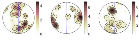
Figure 8. Representative pole figures for crystallographic axes [100], [010] and [001] of olivine (a) and axes or poles [100], (010) and (001) of plagioclase (b) in Wadi Wariyah. The pole figures are arranged by their height in the sequence; text block aside gives the layer number, the depth in the layered sequence, the corresponding BA or BC index, and the ODF J index of the sample. N is the number of analyzed grains. The blue line gives the foliation estimated from (010) of plagioclase. Note the differently scaled color bars.
