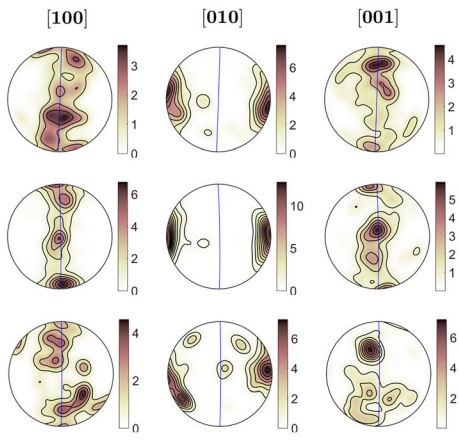
Figure 8. Representative pole figures for crystallographic axes [100], [010] and [001] of olivine (a) and axes or poles [100], (010) and (001) of plagioclase (b) in Wadi Wariyah. The pole figures are arranged by their height in the sequence; text block aside gives the layer number, the depth in the layered sequence, the corresponding BA or BC index, and the ODF J index of the sample. N is the number of analyzed grains. The blue line gives the foliation estimated from (010) of plagioclase. Note the differently scaled color bars.
