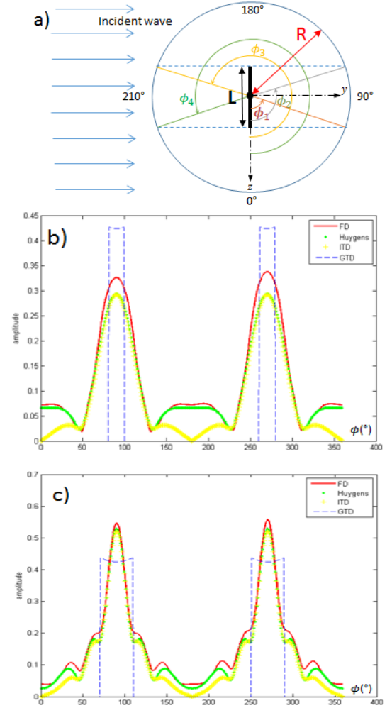
Fig. 5. a) An edge of length L impinged by an incident longitudinal plane wave. Longitudinal edge diffracted field simulated by different models: b) L=10\text{mm} ; c) L=20\text{mm} .
