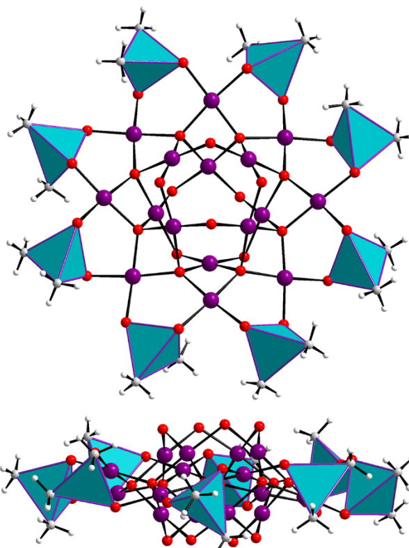
Figure 1. Structural representation of the disk-shaped Pd 16 , top view (top) and side view (bottom). Color code: Pd violet, O red, C grey, H white balls; (CH_3)_2AsO_2 cyan tetrahedra.
