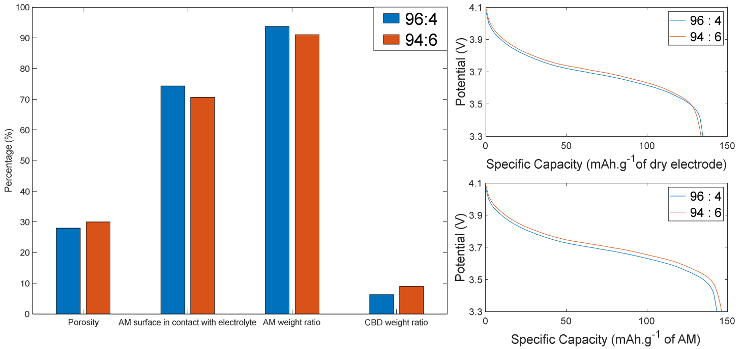
Figure 2. For both electrodes with 96:4 and 94:6 compositions (a) observables from INNOV, discharge curves at 0.8 C with specific capacity per gram of (b) dry electrode and (c) AM. The simulated discharge curves are extrapolated from 3.4 V to 3.3 V.
