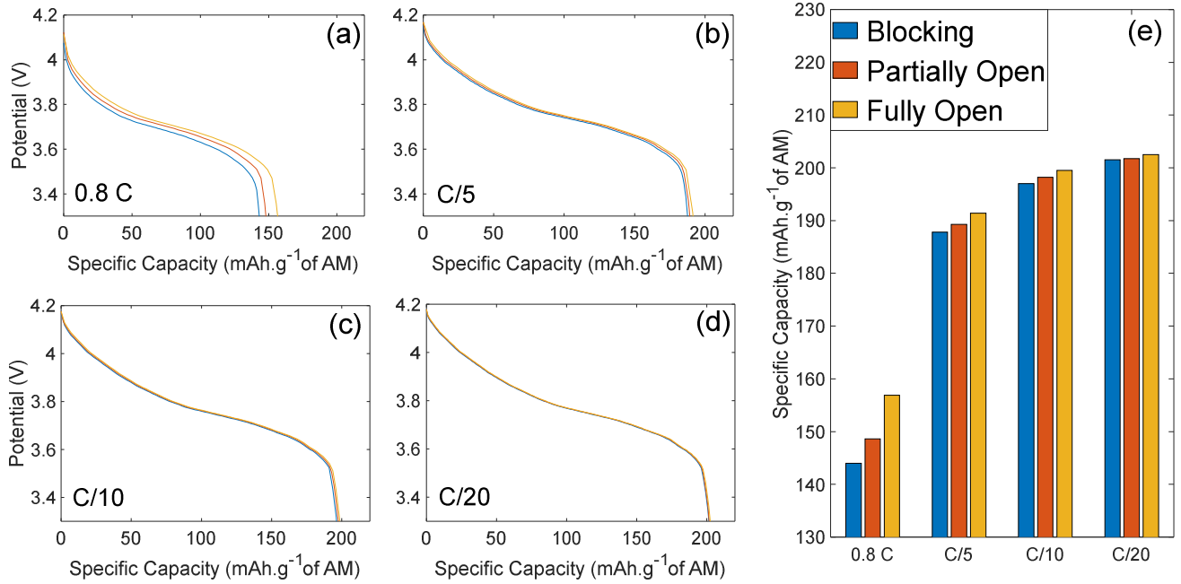
Figure 3. Discharge curves of the 96:4 electrode along the blocking, partially open and fully open assumptions at (a) 0.8 C, (b) C/5, (c) C/10, (d) C/20 and (e) the histogram of the specific capacities at the end of discharge (3.3 V) for each C-rate. The simulated discharges curves that stopped at 3.4 V are extrapolated in order to reach 3.3 V.
