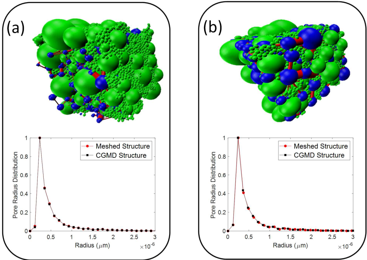
Figure 1. Pore network of the CGMD structure and pore size distribution of the mesh and CGMD structures for (a) 94:6 and (b) 96:4 electrodes. On the image, the solid particles are represented in green, the throats of the percolation network in red and the cavities in blue.
