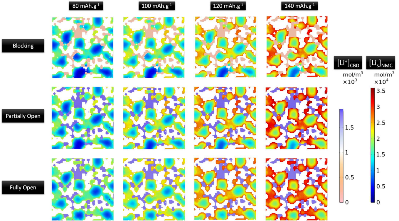
Figure 4. Snapshots at different depths of discharge of the lithium concentration inside the solid phase for a 96:4 electrode for (a) blocking CBD, (b) partially open CBD and (c) fully open CBD hypothesis at 0.8 C.
