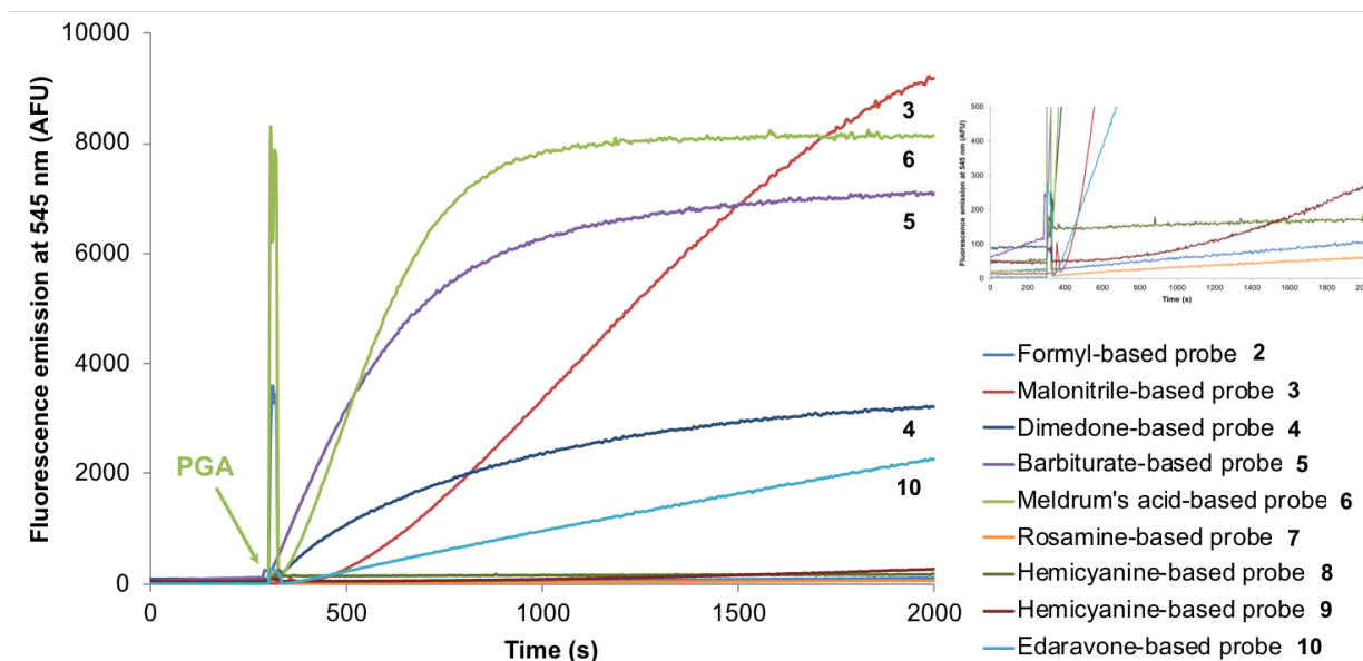
Fig. 2 Time-dependent changes in the green-yellow fluorescence intensity (Ex./Em. 525/545 nm, slit 5 nm) of fluorogenic probes 2-10 (concentration: 1.0 \mu M) in the presence of PGA (1 U) in PB (100 mM, pH 7.6) at 37 ^{\circ} C. Please note: PGA was added after 5 min of incubation of probe in PB alone.
