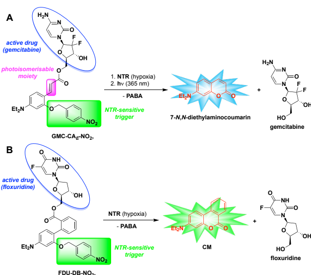
Fig. 4 Hypoxia-activated anticancer theranostic prodrugs based on the "covalent-assembly" strategy and already reported in the literature. 24
