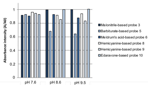
Fig. 6 UV-vis absorbance changes (at \lambda_{\max} ) of fluorogenic probes 3 , 5 , 6 , 8 , 9 and 10 after 30 min incubation in three distinct aq. buffers (PB, 100 mM, pH 7.6 and borate buffer, 100 mM, pH 8.6 and 9.5) at 25 °C (concentration: 2.0 \mu M).
