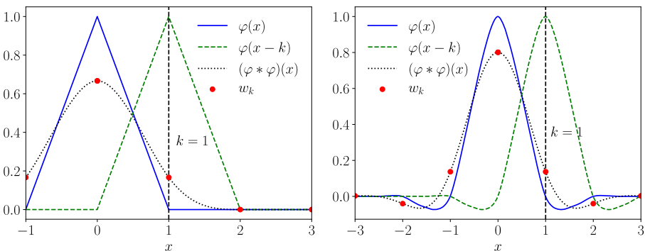
Fig. 18 Autocorrelation functions of Deslauriers interpolating scaling functions \varphi of order two (left) and order four (right)
