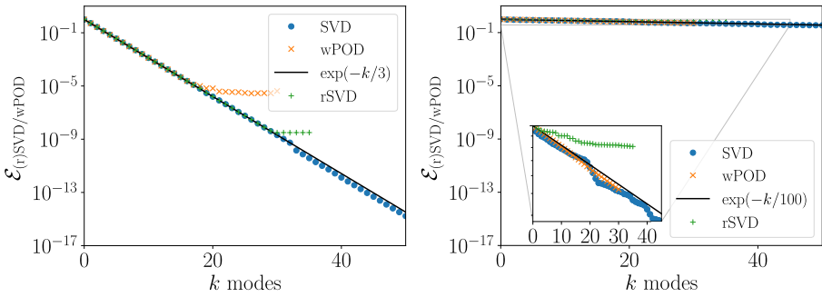
Fig. 9 Comparison of the total approximation errors \mathcal{E}_{(r)SVD}, \mathcal{E}_{wPOD} for \Delta\lambda = 3 (left) and \Delta\lambda = 100 (right). As reference we plot the exact values \exp(-k/3) and \exp(-k/100) indicated by a black line. The rSVD is computed with 35 random samples of \mathbf{U} and the wPOD set up with \epsilon = 6 \times 10^{-3} and J_{\max} = 5 , to ensure approximately the same memory consumption. The inset shows a zoom
