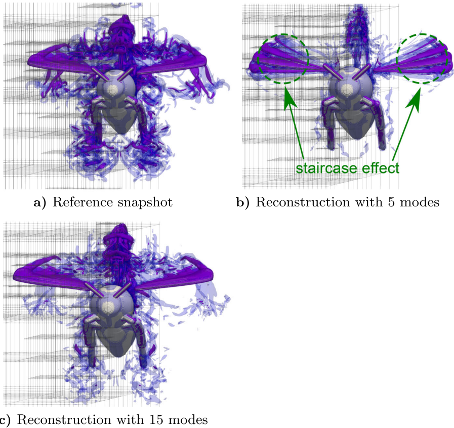
Fig. 14 Comparison between a bumblebee snapshot at time t_i , i = 13 a) and its POD reconstruction \tilde{\mathbf{u}}_i^{\epsilon} using 5 modes b) and 15 modes c) with \epsilon = 0.01 . Shown are two isosurfaces of the magnitude of vorticity, i.e., \|\text{curl}(\mathbf{v})\|_2 = 50 and 100 . The rigid body of the bumblebee is displayed in gray. The grid structure is indicated behind. Staircase effects at the wings are indicated in Fig. 14b. These artifacts appear when POD is applied to sharp structures or discontinuities which move
