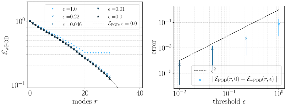
Fig. 16 Total relative error, \mathcal{E}_{wPOD} , of the wPOD (left) and difference of the wPOD and POD error, \Delta\mathcal{E}(r, \epsilon) = |\mathcal{E}_{POD}(r, 0) - \mathcal{E}_{wPOD}(r, \epsilon)| (right). The error bars in the right figure indicate the minimal and maximal value of \Delta\mathcal{E} for all ranks 1 \leq r \leq 30 and the markers the mean \overline{\Delta\mathcal{E}}(\epsilon) = 1/30 \sum_{r=1}^{30} \Delta\mathcal{E}(r, \epsilon)
