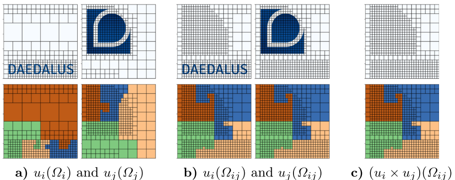
Fig. 4 Visualization of pointwise operations on multiresolution grids \Omega_i and \Omega_j . On the top row the scalar fields u_i and u_j are shown, where blue colors represent 1 and white colors 0. Below each field the corresponding processor distribution grid is displayed. Each color of the processing grid represents one of the four processing units. Initial trees (Fig. 4a), unified tree structures (Fig. 4b) and the processed field (Fig. 4c)
