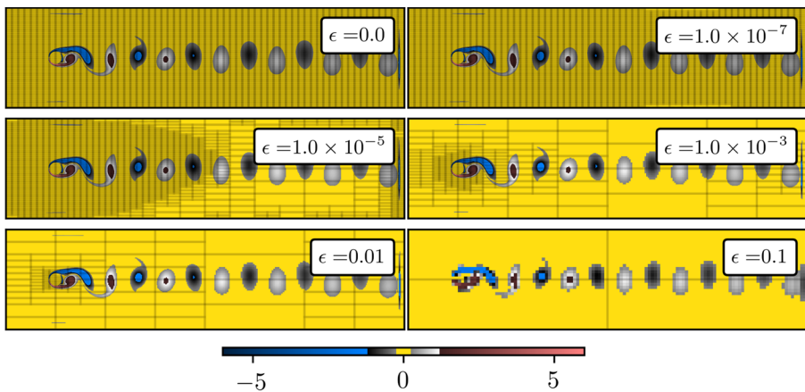
Fig. 3 Block-based adaptation of a flow past a cylinder for different thresholds \epsilon . Shown is the vorticity field \omega^\epsilon = \partial_x v_y^\epsilon - \partial_y v_x^\epsilon , which is computed after having applied the wavelet adaptation to the full state vector \mathbf{u}^\epsilon = (v_x^\epsilon, v_y^\epsilon, p^\epsilon) . Each block represents B_1 \times B_2 = 65 \times 17 points. More details can be found in Section 4.2.1
