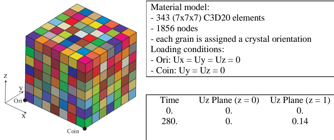
Fig. 2. Simplified RVE for the first step of the identification. Each finite element represents a crystal.
