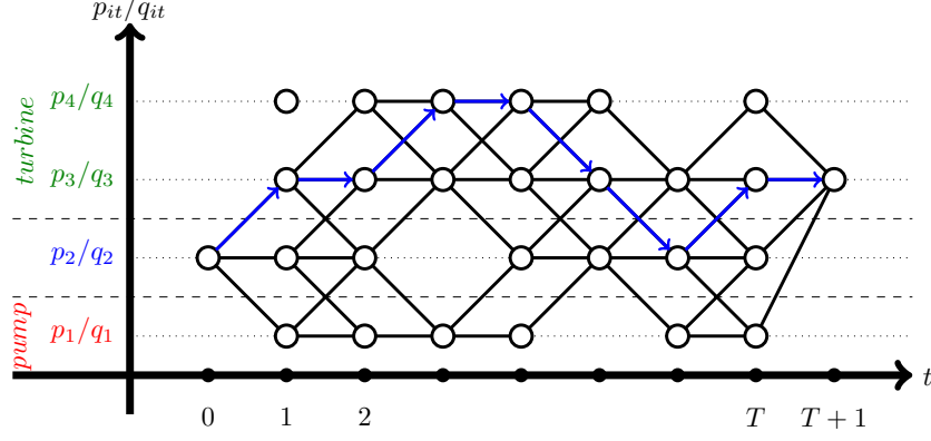
Figure 1: G = (N, A)
