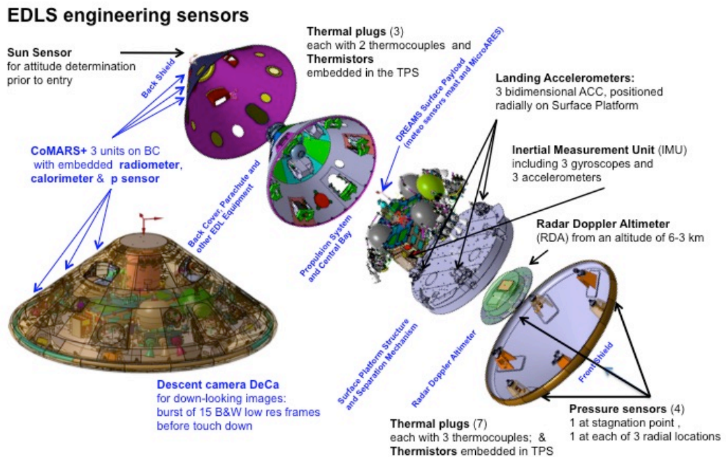
Fig. 2: ExoMars2016 Schiaparelli Entry and Descent Module and EDL engineering sensors (credit: ESA, TAS-I, readapted)
