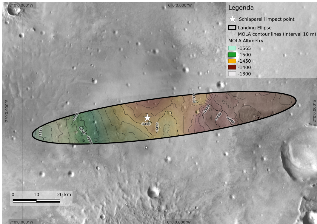
Fig. 8 ExoMars2016 Schiaparelli landing site in Meridiani Planum. The landing ellipse, centred at 6^{\circ} West and 2^{\circ} South, measured about 100 km East-West and 15 km North-South. It was located on a relatively smooth, flat region as evidenced by the overlaid topographic map (source data: Mars Odyssey - THEMIS Day-IR, MGS – MOLA). The actual Schiaparelli impact site, as detected in the MRO HIRISE images, is marked with a star. (Credit: IRS/PS/TAS-I/ESA).
