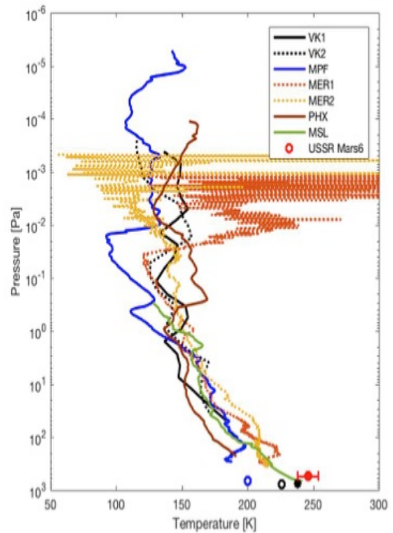
Fig. 3 Mars atmospheric profile as measured by entry probes.
