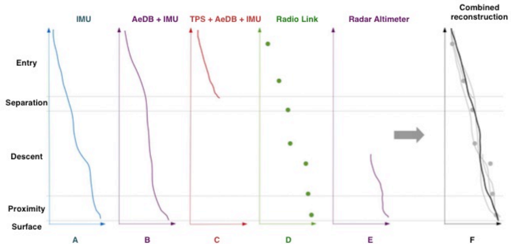
Fig. 5 A schematic view of the AMELIA reconstruction approach. (A) Starting from the direct numerical integration of IMU data velocity, position and attitude are derived. (B) The aerodynamical data base (AeDB) is used in order to convert the sensed accelerations into atmospheric parameters; outputs are velocity, position, angle of attack (AoA), side slip angle (SSA) which give the density, pressure and temperature profiles. (C) IMU aided TPS pressure data processing provides the static and dynamic pressures which give density and temperature profile. (D) From the Doppler shift of the radio link received on ground and via the Mars Relay orbiters, it is possible to measure the EDM velocity in Line-of Sight and to derive position, and possibly winds. (E) The EDM radar altimeter provides a direct measurement of the EDM elevation with reference to the Mars ground. (F) The combined reconstruction is assessed by checking the agreement of the different techniques, using data assimilation and by Extended Kalman filtering.
