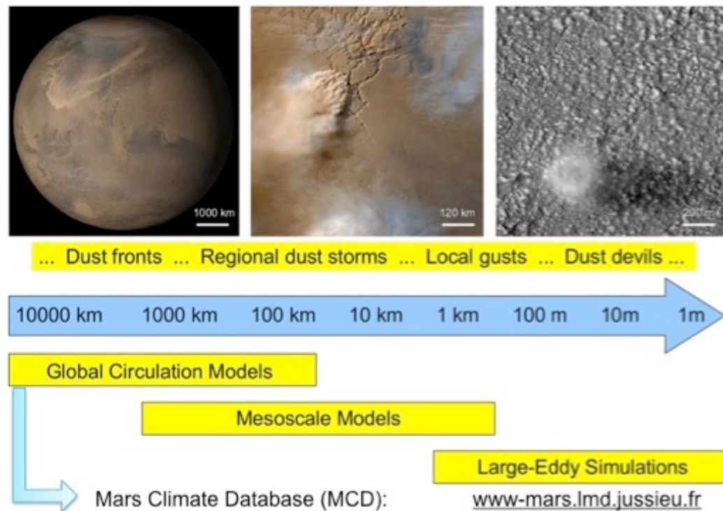
Fig. 6 Tools to model Mars' environment. Typical Mars weather events related to dust lifting (top images + yellow strip), relevant spatial scales (middle blue arrow) and meteorological models for their analysis (bottom yellow strip) are reported. The outputs of the integrated models have been implemented into the Mars Climate Database (MCD www-mars.lmd.jussieu.fr ) in order to forecast the mean environmental parameters at a specific place, season, time of the day, and altitude. Image credits, left: NASA-MGS-MOC, middle: NASA-MRO-MARCI, right: NASA-MRO-HIRISE; images retrieved from the NASA Planetary Data System PDS: Figure from Spiga and Lewis, 2010, modified with permission.
