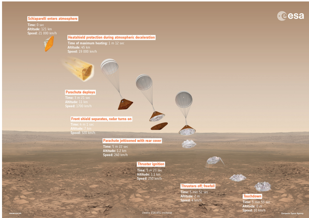
Fig. 1: ExoMars2016 Schiaparelli EDL scenario (credit: ESA) The sequence of entry, descent and landing of the Schiaparelli EDM and relevant events are reported together with the expected timing, altitude and velocity, as simulated for the reference mission using forecast atmospheric scenarios.
