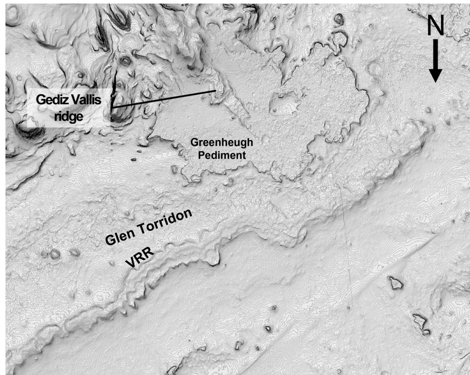
Figure 17. A 1 m contour map emphasizing topographic relationships between Vera Rubin ridge (VRR), Glen Torridon, and the Greenheugh pediment and unique shape of VRR.
