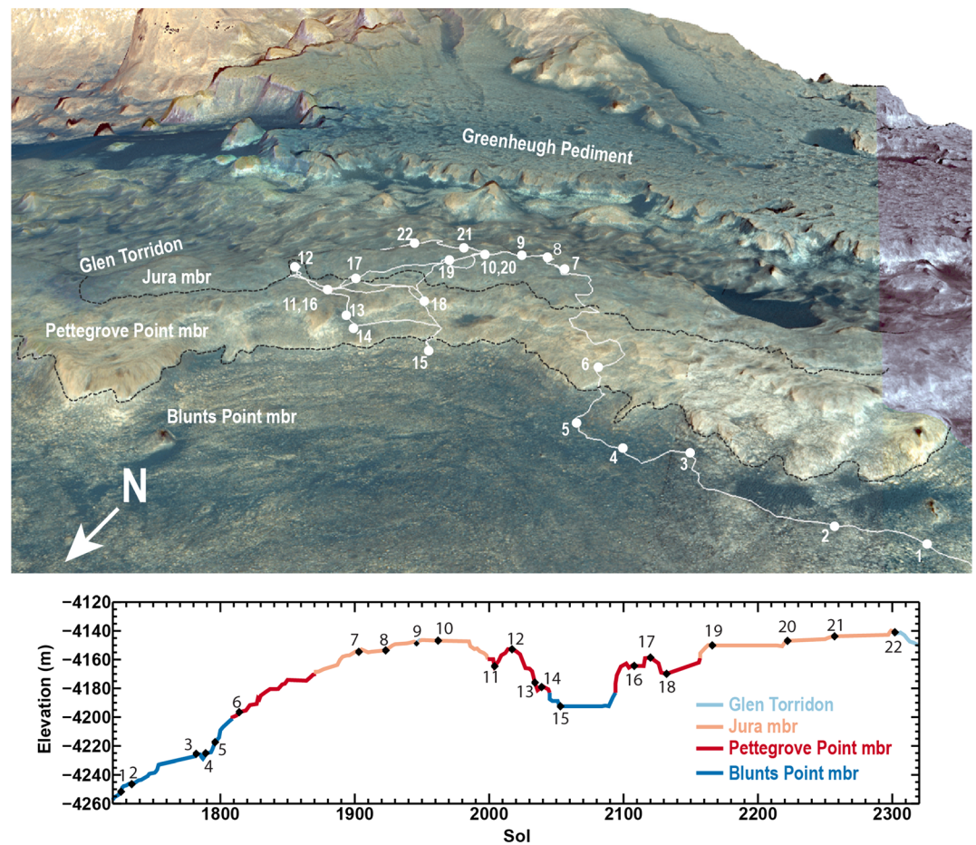
Figure 4. (top) Perspective view of Curiosity's traverse over VRR with stratigraphic members and key campaign stops labeled. (bottom) Sol versus elevation along traverse. Numbered stops key: (1–5) approach imaging stops, (6) fracture investigation, (7, 8) first gray patch investigation, (9) toe dip into Glen Torridon unit, (10) Lake Orcadie rotary-only drill attempt, (11) reconnaissance of area with strongest CRISM spectral signature, (12) Bressay deposit investigation, (13) Taconite crater, (14) Red Cliff imaging stop, (15) Blunts Point drill, (16) Voyageurs failed drill, (17) Ailsa Craig failed drill, (18) Stoer drill, (19) Inverness failed drill, (20) Highfield drill, (21) Rock Hall drill, and (22) transition to Glen Torridon.
