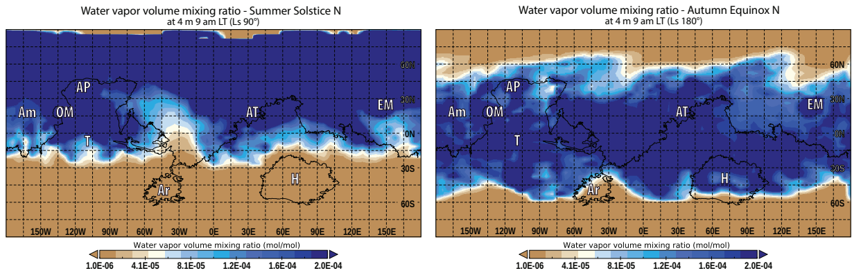
Figure 11: Global distribution of water vapor volume mixing ratio at 9 am LT derived from GCM at the time of the northern summer solstice (left) and northern autumn equinox (right). According to the daily curves, the VMR returns to the daytime levels by this time. In the map we can see, that indeed the water vapor above the surface is mostly continuous in distribution with values around 1.6 \times 10^{-4} mol/mol in both seasons presented here.
