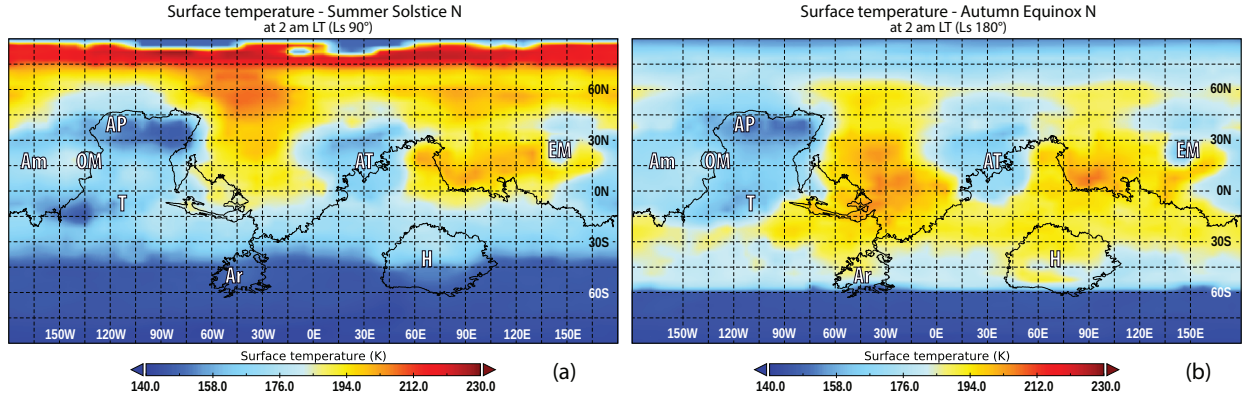
Figure 7: Seasonal dependence of the nighttime surface temperatures data from GCM at the time of the northern summer solstice (a) and northern autumn equinox (b), 2 am LT everywhere. The three “humid” zones defined in section 3 are apparent here, these are approximately 30 K colder than their surroundings. The area east of Alba Patera (AP) seem the coldest part of these three zones, being an extra 10 K lower in temperature than the rest of the previously defined “humid” regions.
