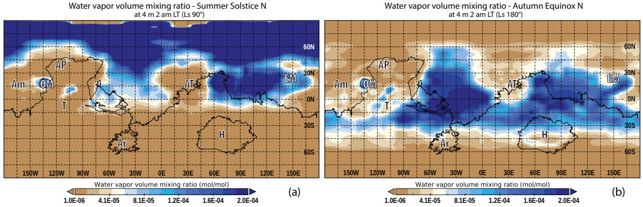
Figure 8: Seasonal dependence of water vapor volume mixing ratio data from GCM at the northern summer solstice (a) and northern autumn equinox (b) at approximately 4 m above surface, 2 am LT globally. The three humid zones defined in Section 3 appear here as regions, where the VMR is approximately 3 orders of magnitude lower than their surroundings. The exceptions are Olympus Mons (OM), Tharsis Montes (northwest from Tharsis denoted by T), and Elysium Mons (EM). These mountains show 1-2 orders of magnitude higher VMR values than the rest of the humid zones. We can also observe, that during northern summer the southern borders of these zones are not defined, with the exception of Arabia Terra (AT). During northern autumn the northern boundaries blend together with the northern polar region. This shows a trend of higher VMR values moving to the south as the seasons change from summer to eventually winter in the Northern Hemisphere (Smith, 2002, Steele et al., 2014).
