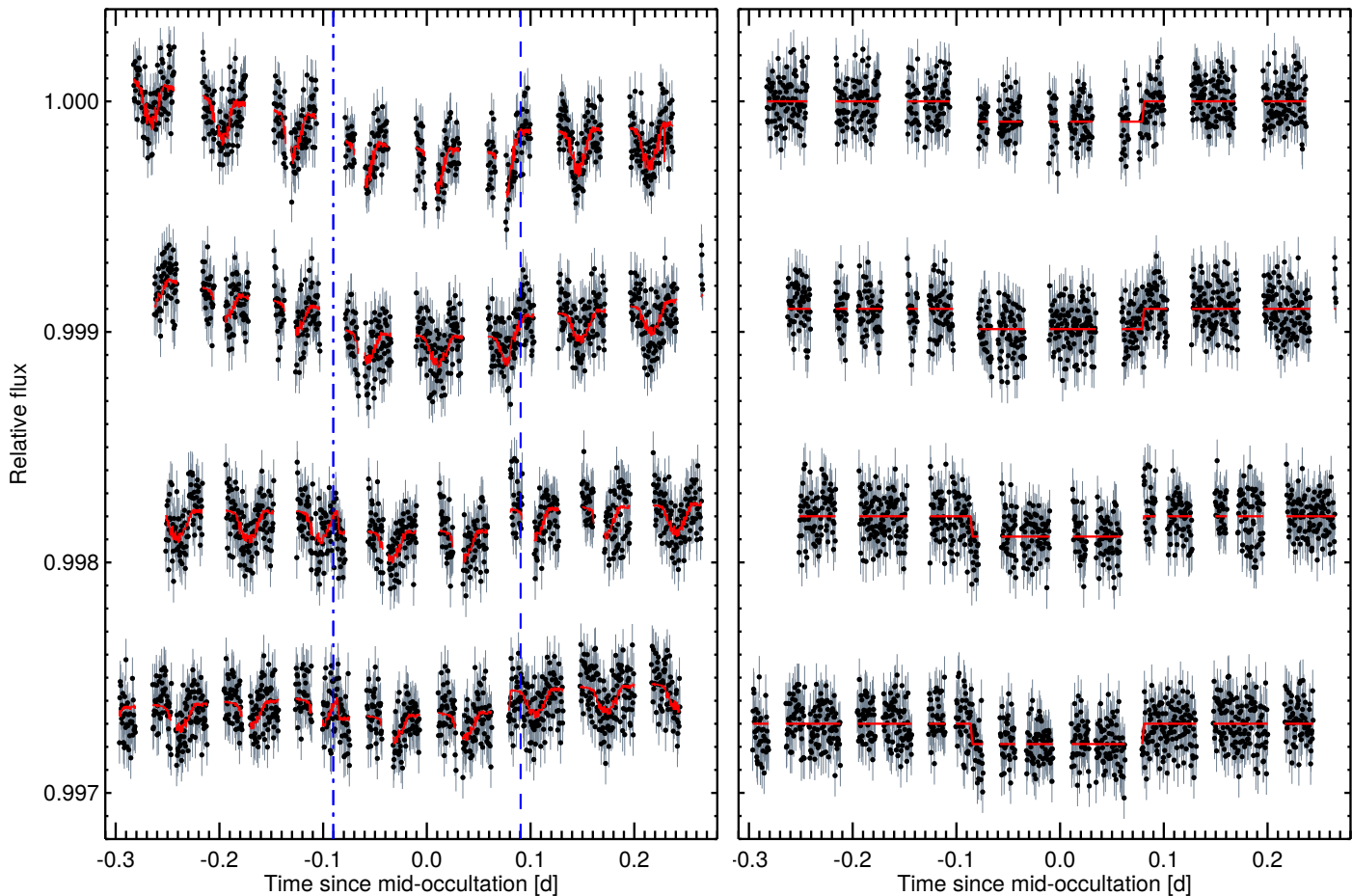
Fig. 1. Individual CHEOPS observations of four WASP-189 b occultations. In both panels, visits are shown chronologically from top to bottom, occurring on 19, 27, and 30 March and 7 April 2020, respectively. Left : uncorrected observations (black points) together with their full (baseline and occultation, red line) light-curve models. Blue vertical dash-dotted lines indicate the beginning and end of occultation. Right : data (black points) corrected for the instrumental and stellar trends, together with the occultation model (red line).
