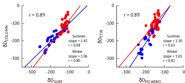
Figure 14. Comparison of columnar \delta D_{\text{v}} vs. \delta D_{\text{v}} at surface: ECHAM5-wiso averaged using Eq. (2) \delta D_{\text{v}} vs. ECHAM5-wiso \delta D_{\text{v}} at surface (left panel), and FTIR retrievals compared to \delta D_{\text{v}} measured by Picarro instrument at surface (right panel).
