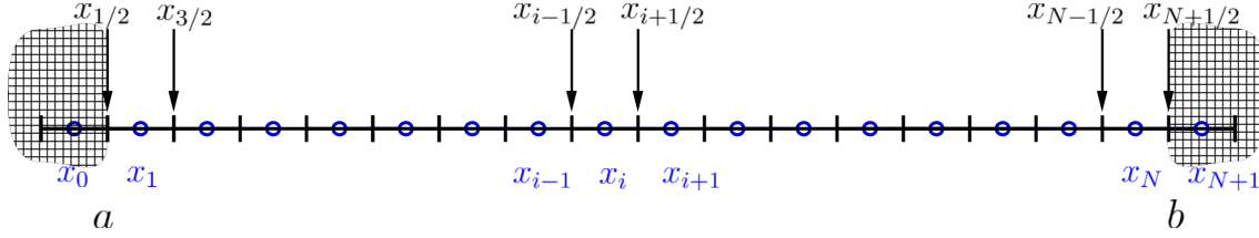
FIGURE 1. Schematic representation of the staggered grid
