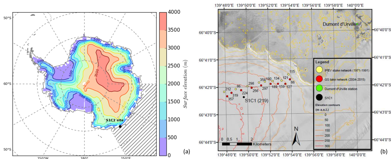
Figure 1. Maps showing the areas of interest with (a) a map of Antarctica representing the local topography (contours), the location of the S1C1 drilling site and the area used to extract regional sea-ice extent from the Nimbus-7 Scanning Multichannel Microwave Radiometer (SMR) and Defense Meteorological Satellite Program Special Sensor Microwave/Imagers - Special Sensor Microwave Image/Sounder (DMSP SSM/I-SSMIS) passive microwave data (hatched area), and (b) an orientation map showing stake networks around S1C1 drilling site. Data from 1971 to 1991 were measured by IPEV, whereas data from 2004 to 2015 were measured in the framework of GLACIOCLIM-SAMBA (GS) observatory. Elevation lines are from the digital elevation model by Korona et al. (2009), which was computed from SPOT5 images obtained during the fourth International Polar Year (2007–2009). The SPOT5 image is also included as a background map. Labels are mean accumulation values at each stake computed over the period with measurements.
