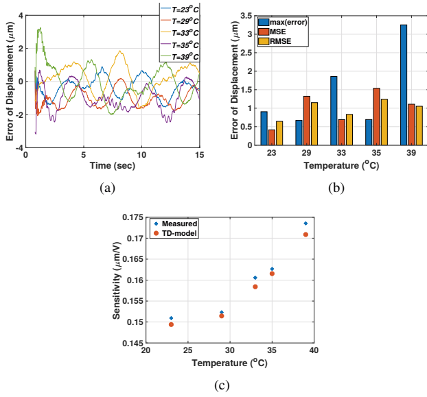
FIGURE 8. (a) Error signal between the measured output displacement and the proposed hysteresis model output using threshold number n = 9 at different environmental temperatures, (b) Maximum error, Mean square error (MSE) and Root mean square error (RMSE) for the measured output displacement and the proposed model hysteresis output, and (c) comparison of the sensitivity of the measured data and the proposed hysteresis model.
