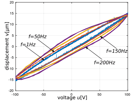
Fig. 4: Experimental hysteresis at different frequencies.
