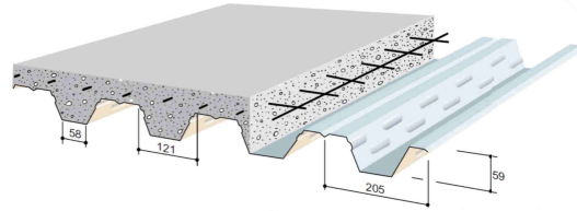
FIGURE 2 – Schematic representation of a Haircol ® slab [16]
