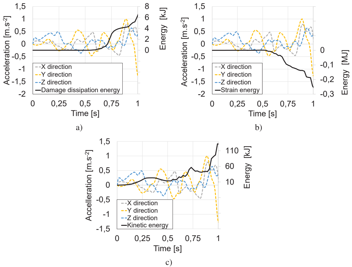
FIGURE 9 – Accelerations data along X, Y, and Z directions and evolution of energies within the model in function of time : (a) damage energy dissipation, (b) strain energy and (c) kinetic energy
