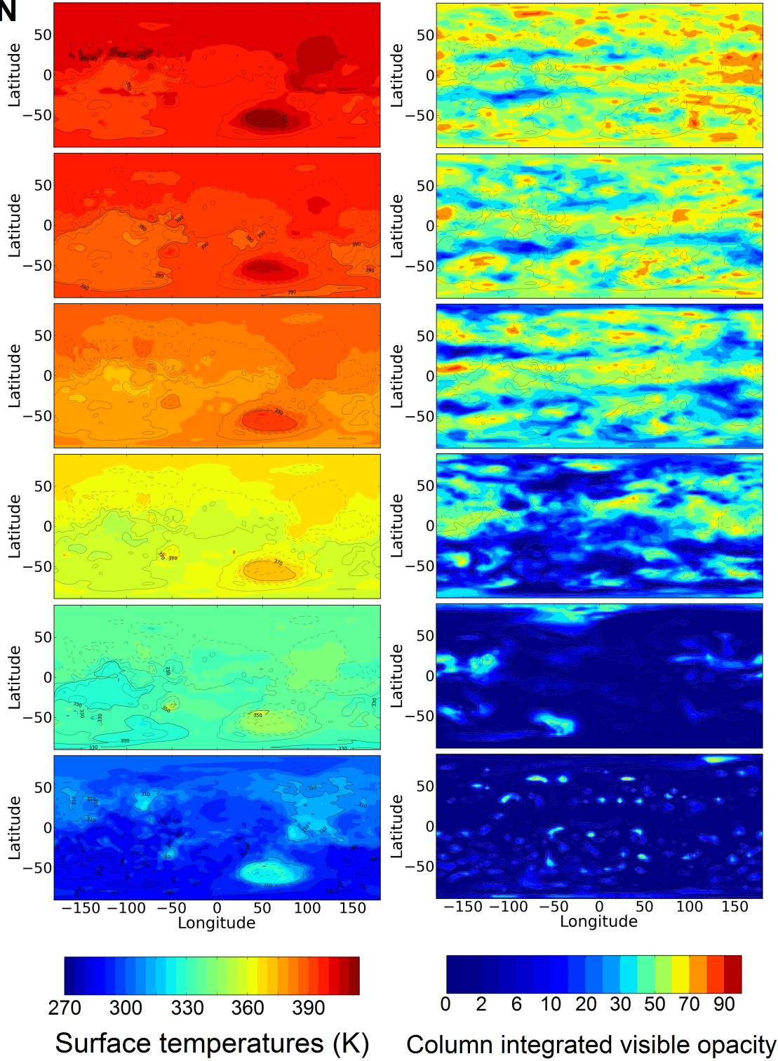
Figure 2: Snapshots of post-impact surface temperature (in K) and visible opacity maps at six distinct timings (1, 3.5, 7, 11, 13 and 14 martian years). These six timings are also highlighted in Fig. 1AF with dots.
