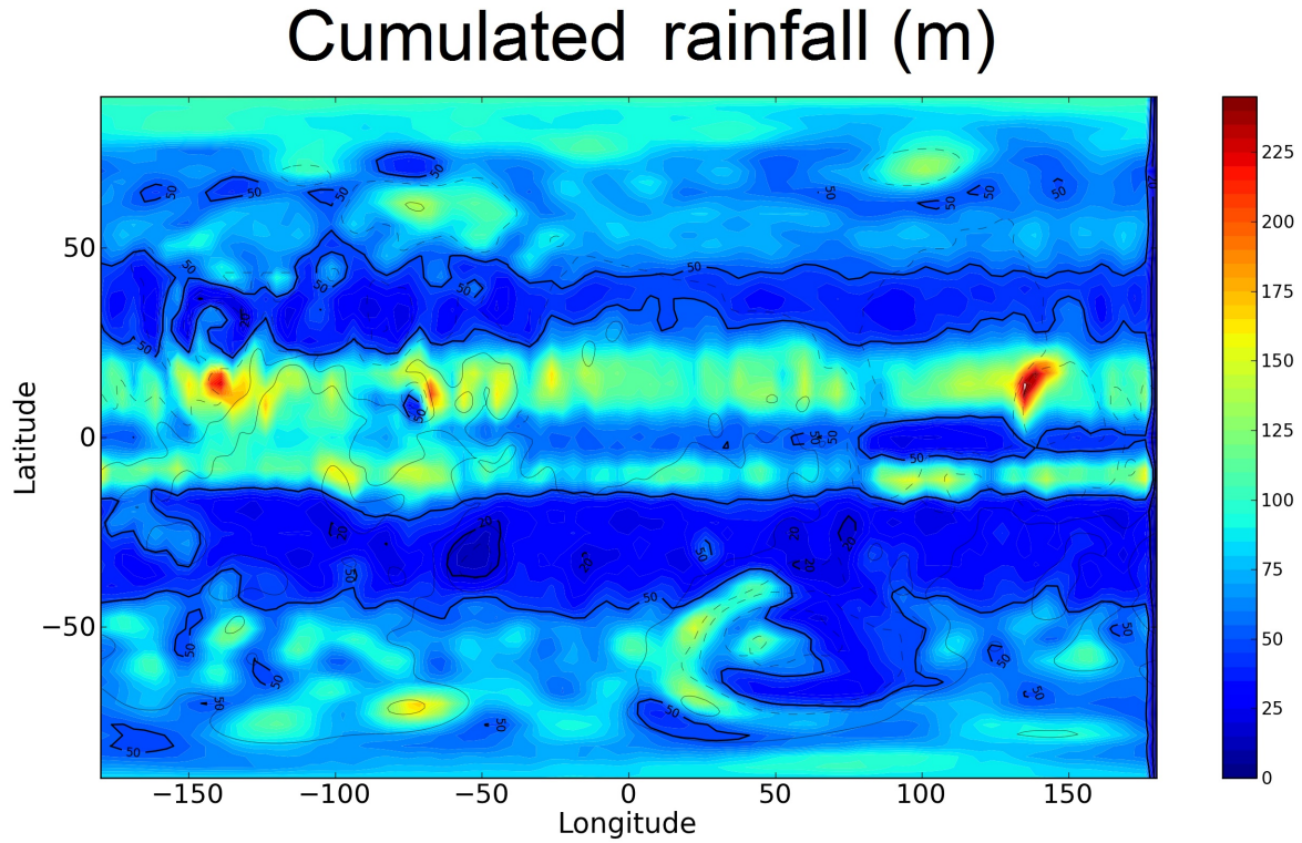
Figure 6: Cumulative rainfall map (in m) 15 martian years after the bolide impact event. Ascending branches of the Hadley cells lie near the equator, while descending branches are located around \pm 30^\circ latitude. The absence of rain at the equator is due to the presence of equatorially trapped modes producing westerly winds.
