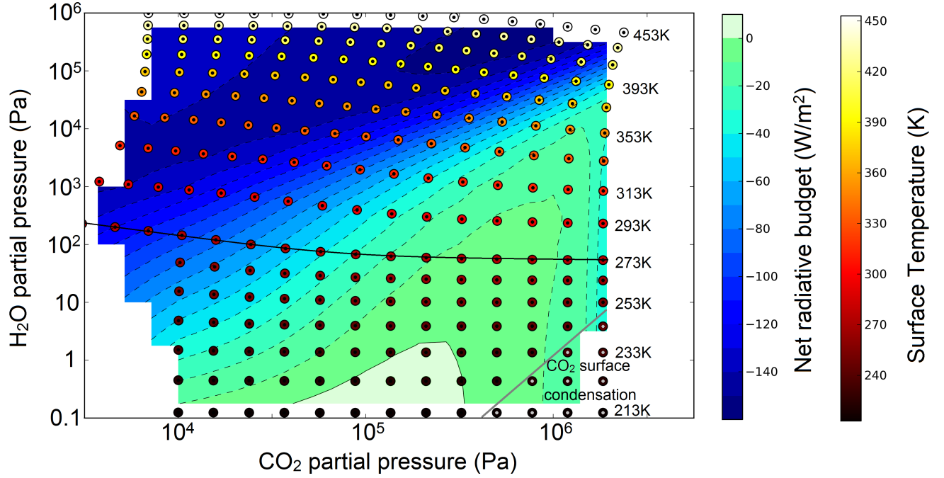
Figure 7: Contour plot of the net radiative budget at the TOA (Top Of Atmosphere) of the post-impact early Mars atmosphere, as a function of \text{CO}_2 and \text{H}_2\text{O} partial pressures in the atmosphere. The contour plot was calculated by interpolating the data points of the scatter plot. The color of the data points corresponds to the surface temperature of the simulation. The planet is at equilibrium if the radiative budget is equal to 0, which is never the case for any of the post-impact simulations. For a given \text{CO}_2 atmospheric content, the increase in \text{H}_2\text{O} content leads to a decrease in the net TOA radiative budget despite the greenhouse effect of water vapour. This is due to the fact that the surface temperature also increases, which increases the OLR and decreases the net radiative budget at the TOA. This dependency stops when the OLR reaches its asymptotic value.
