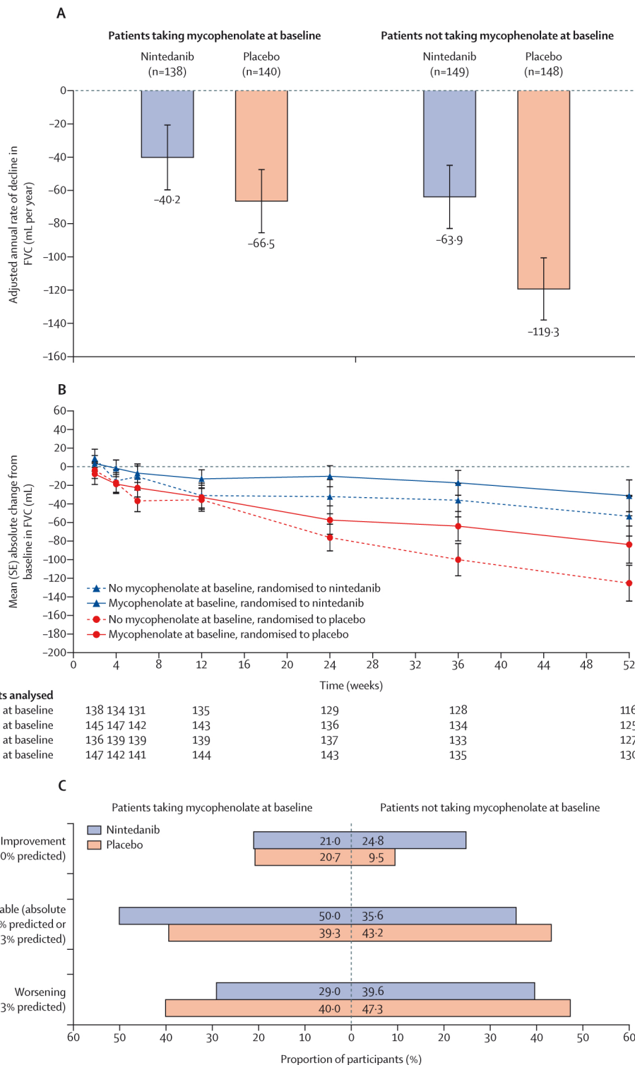
Figure 2: Annual rate of decline in FVC (mL per year) over 52 weeks (A), observed change from baseline in FVC (mL) over 52 weeks (B), and proportion of participants who had improvement in FVC, stable FVC, and worsening of FVC between baseline and week 52 (post-hoc analysis; C), in subgroups by use of mycophenolate at baseline. In part A, random coefficient regression model including anti-topoisomerase I antibody status, age, height, sex, and baseline FVC (mL) as covariates and terms for treatment-by-subgroup and treatment-by-subgroup-by-time interaction. p value for treatment-by-time-by-subgroup interaction was 0.45. 138 of 139 participants in the nintedanib group who were taking mycophenolate at baseline were analysed; a post-baseline FVC measurement was not available for one patient. In panel C, analysable population was 138 in the nintedanib group taking mycophenolate at baseline and 149 not taking mycophenolate at baseline, and 140 in the placebo group taking mycophenolate at baseline and 148 not taking mycophenolate at baseline. Patients with improvement in FVC: p=0.011 for treatment-by-subgroup interaction; patients with worsening of FVC: p=0.62 for treatment-by-subgroup interaction. FVC=forced vital capacity.
