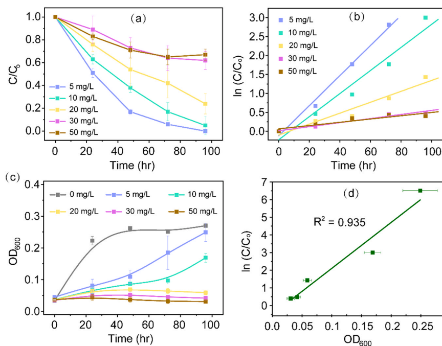
Fig. 1. Time course of the removal of chloramphenicol by G. sulfurreducens PCA under different initial concentrations (a) and kinetic fitting (b) at 30^\circ\text{C} . The \text{OD}_{600} values of G. sulfurreducens PCA at five initial chloramphenicol concentrations (c) and the relevance to \ln(C/C_0) (d). Values are the mean of three biological replicates. Error bars represent the SD.
