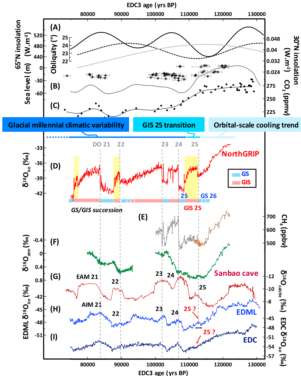
Figure 1. (a) 65^{\circ}\text{N} insolation (black), 30^{\circ}\text{N} insolation (grey) and obliquity (dashed black) [Laskar et al., 2004]. (b) Sea level relative to present, reconstructions from Bintanja et al. [2005] (grey curve) and Thompson and Goldstein [2005] (black crosses with associated uncertainties). (c) \text{CO}_2 data [Lüthi et al., 2008], smoothed curve (black) produced from a five-point binomial filter using 1200-yr resampled data. (d) NorthGRIP \delta^{18}\text{O}_{\text{ice}} [NorthGRIP Community Members, 2004]. GIS beginning is marked by an abrupt warming referred to as DO. Yellow boxes indicate rebound-type structures: GIS 22, GIS 25 and the rapid event ending GIS 21 [Capron et al., 2010a]. (e) NorthGRIP \text{CH}_4 grey triangle: Capron et al. [2010b]; this study: red triangle. (f) NorthGRIP \delta^{18}\text{O}_{\text{atm}} [Landais et al., 2010]. (g) \delta^{18}\text{O}_{\text{calcite}} of Sanbao Cave speleothems [Wang et al., 2008]. (h) EDML \delta^{18}\text{O}_{\text{ice}} [Stenni et al., 2010]. Antarctic Isotopic Maximum events are indicated (AIM). (i) EDC \delta^{18}\text{O}_{\text{ice}} . Jouzel et al. [2007] and Stenni et al. [2010] have suggested that an Antarctic counterpart of DO 25, named AIM 25, was visible in \delta^{18}\text{O}_{\text{ice}} profiles from the EPICA ice cores: the millennial-scale event identified as AIM 25 is indicated for each record by the red arrow. The associated question marks illustrate that such identification remains equivocal. Except for the Sanbao \delta^{18}\text{O}_{\text{calcite}} record, the orbital parameters, and the sea level reconstruction from Thompson and Goldstein [2005], records are synchronised on the EDC3 timescale [Parrenin et al., 2007; Capron et al., 2010b]. Dashed light pink lines indicate rapid event onsets. The black arrow indicates the temporal uncertainty linked to the timescale synchronisation at the onset of GIS 25. The horizontal bar indicates the GIS/GS succession and dots indicate the ambiguity that remains on defining the start of GS 26 and GS 23.
