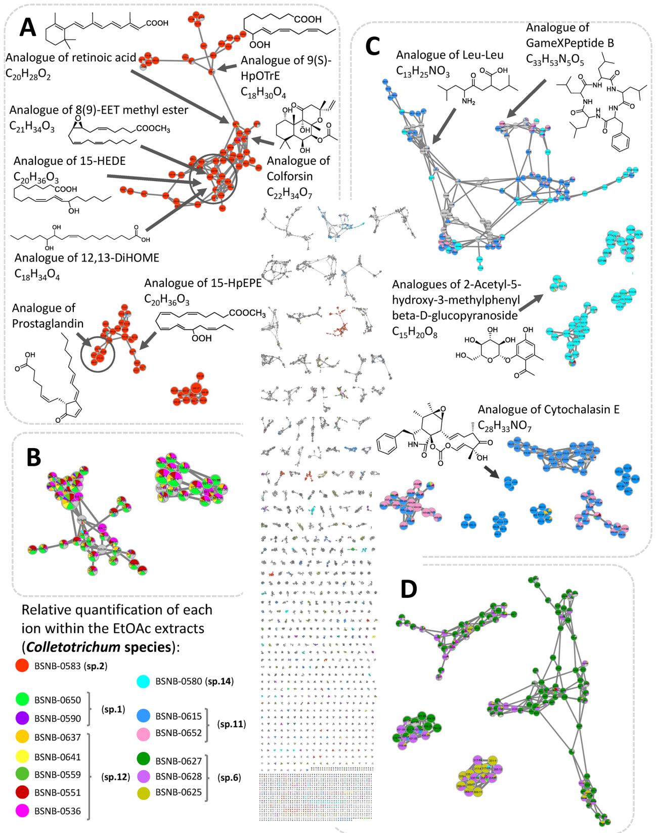
Figure 2. Massive molecular network of the 42 extracts from Astrocarylum sciophilum endophytes. MN is reduced to the ions with m/z between 200 and 900 and the selfloop nodes were removed to give a MN of 6316 nodes. Boxes (A–D) regroup clusters of ions from the MN: Relative quantification of each ion was represented as pie chart diagrams, the proportions of which were based on respective areas of the corresponding extracted ion chromatogram (XIC) area. MetGem software ( https://metgem.github.io/ ).
