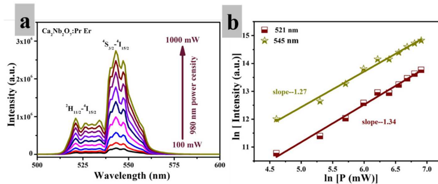
Fig. 5. (a) The upconversion emission spectra of the \text{Ca}_2\text{Nb}_2\text{O}_7:\text{Pr}/\text{Er} sample with different pumping powers under 980 nm excitation. (b) The upconversion emission intensity at 521 and 545 nm versus pumping powers for the \text{Ca}_2\text{Nb}_2\text{O}_7:\text{Pr}/\text{Er} sample.
