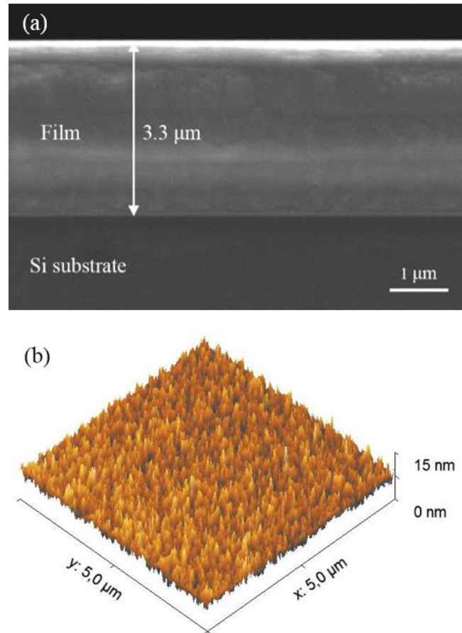
Fig. 1. (a) The cross sectional SEM image and (b) 3D AFM morphology of the Ti16132 film deposited on Si (100) substrate.
