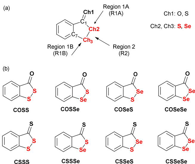
Scheme 1. (a) Possible \sigma -hole Regions around the Dichalcogenide Ch2–Ch3 Bond in the 1,2-Dichalcogenole series (b) Molecular Structures of Investigated Compounds.
