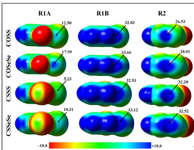
Figure 5: ESP maps of COSS, COSeSe, CSSS and CSSeSe drawn along R1A, R1B and R2 \sigma -hole regions. ESP is mapped on the molecular \rho = 0.002 a.u. isosurface. Blue: positive, Red: negative. ESP values in the figure are reported in kcal/mol. See Figure S10 for others compounds.
