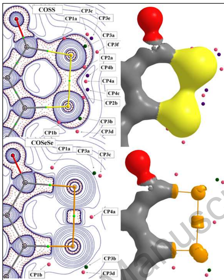
Figure 6. Left: L(\mathbf{r}) = -\nabla^2\rho(\mathbf{r}) maps [ e/\text{\AA}^5 , contours are in logarithmic scale: positive (red) and negative (blue)] for COSS (top) and COSeSe (bottom). Right: The \nabla^2\rho(\mathbf{r}) = 0 maps are plotted for COSS (top) and COSeSe (bottom) with atomic portioning. Relevant CPs of L(\mathbf{r}) in the valence shell of chalcogen atoms are denoted in maps as spheres [(3, -1) CPs are green, (3, +1) CPs are pink and (3, +3) CPs are violet]. (3, -3) CPs corresponding to lone-pairs of Ch2 and Ch3 are out of plane in the left (they are shown in Figure S13), and hidden by the enclosing surfaces \nabla^2\rho(\mathbf{r}) = 0 in the right. See Figures S14–S16 for other compounds.
