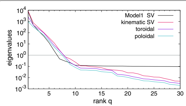
Fig. 15 The eigenvalue spectra of the classical, kinematic secular variation, toroidal and poloidal flow variability, respectively. The horizontal line marks eigenvalues equal 1
