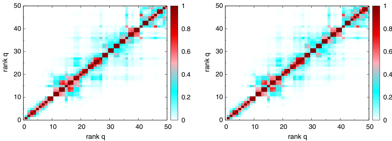
Fig. 14 The weighted correlation matrix. Red colors represent stronger correlation between eigenvectors and therefore a weaker separation. The color scale corresponds to absolute values of correlations from 0 (white) to 1 (dark red)
