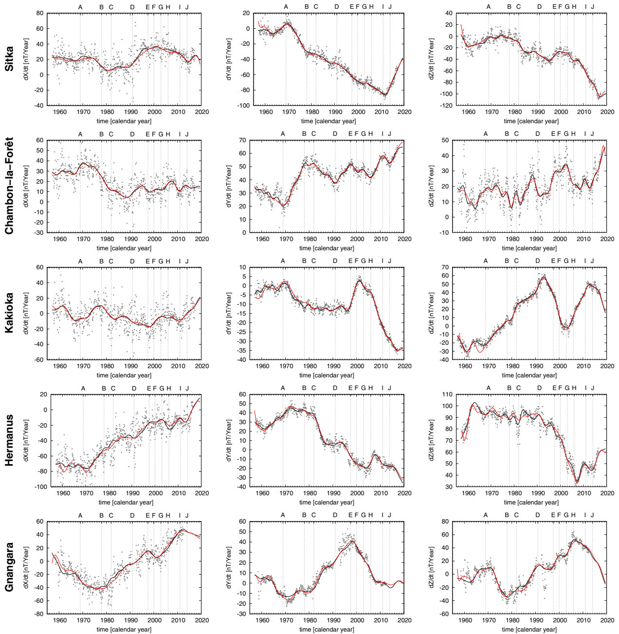
Fig. 3 Observed and modeled secular variation at some observatory sites. From top to bottom: Sitka (Alaska), Chambon-la-Forêt (France), Kakioka (Japan), Hermanus (South Africa), Gngangara (Australia). The gray dots represent the observed monthly secular variation in X, Y and Z (from left to right). Solid curves display the modeled secular variation of Model 1 (black) and Model 2 (red). Vertical lines mark occurrences of geomagnetic jerks
