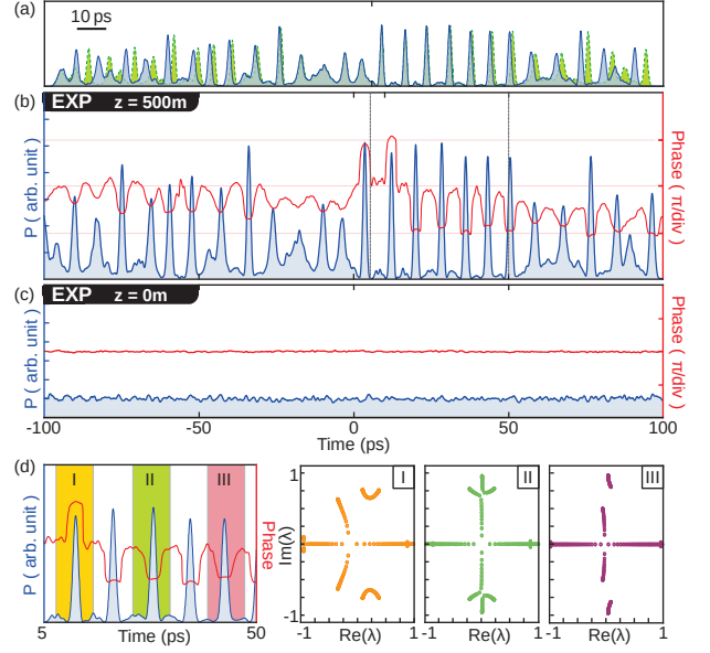
Fig. 3. Experimental complex fields recorded and reconstructed (c) before and (b) after propagation in 500 m of single-mode fiber. (a) shows the reconstructed intensity of the same field with (solid blue line) and without (dashed green line) compensation of the aberrations. (d) (left panel) Focus on the quasi-periodic pattern of (b) and (right panels) periodic IST profiles of isolated structures. Parameters are the same as in the caption of Fig. 2.
