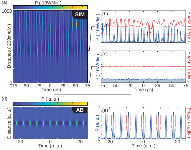
Fig. 2. Typical numerical simulation of the NLSE exhibiting noise-driven MI. (a) Spatio-temporal diagram of the intensity for the first 1000 m of propagation. Complex field at (c) the initial state and (b) after 420 m of propagation. P_0 = \langle |\Psi(z=0)|^2 \rangle = 6W , \beta_2 = -20 \text{ ps}^2/\text{km} , \gamma = 1.3/W/\text{km} . (d, e) Same layout as previously but for an exact AB solution. The dashed red line in (e) is the phase of the AB just after the maximum compression. Parameter for the AB is a = 0.25 according to notation in Ref. [20].
