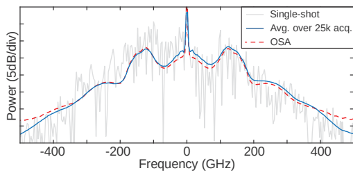
Fig. 4. Single-shot Fourier spectrum computed from the complex field of Fig. 3(b) along with the average spectrum computed over 25 000 single-shot acquisitions and a trace from an optical spectrum analyzer (OSA) recorded simultaneously.
