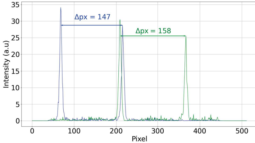
Fig. S1. Double pulse recorded by using the SEAHORSE. The separation \Delta px between the two pulses recorded on the camera depends on their mean position \langle px \rangle within the measurement window. Blue and green curve are two different snapshots.
