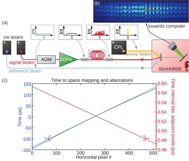
Fig. 1. (a) Schematic description of the experimental setup. (b) Example of a single-shot recording in false colors. (c) Mapping of the time on the horizontal axis of the camera taking account (solid blue line) or not (dashed blue line) of the cubic contribution to the phase of the pump pulses (red line is the derivative of the solid blue line). cw: continuous wave, AOM: acousto-optic modulator, EDFA: Erbium-doped fiber amplifier, CPL: chirped pulse laser
