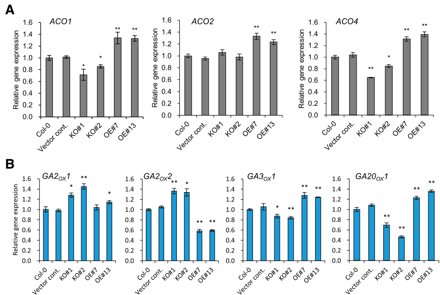
Figure 7. The mRNA levels of ethylene and GA biosynthesis genes in pPLAIII \alpha -OE lines. A and B, Gene expression patterns of ACOs (A) and of gibberellin oxidases ( GA2ox1 , GA2ox2 , GA3ox1 , and GA20ox1 ; B) from control, KO , and OE seeds imbibed for 20 h. Mean \pm SE (SE) of three independent replicates. Asterisks indicate significant difference using Student's t test (* P < 0.05 and ** P < 0.01) compared with the controls.
