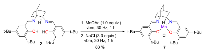
Scheme 2. Mechanochemistry of Mn(III) salen complex 7 .
